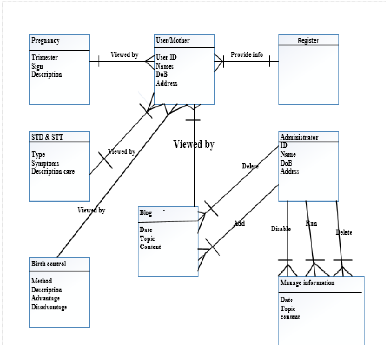
Figure 7: Partial Domain Model
