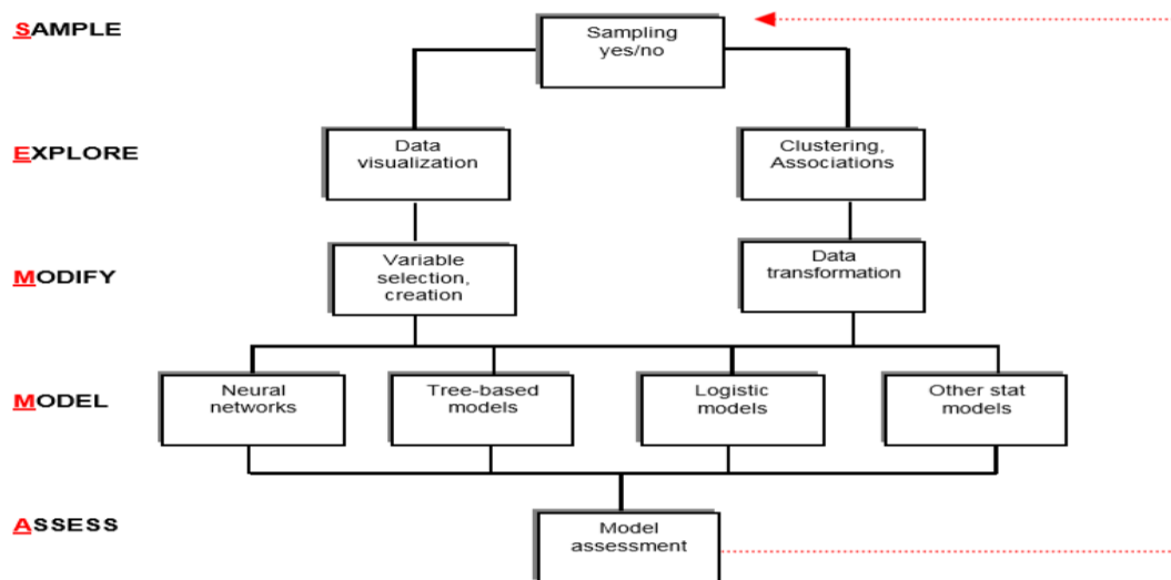
FIGURE 2.2: The SEMMA Analysis Cycle
