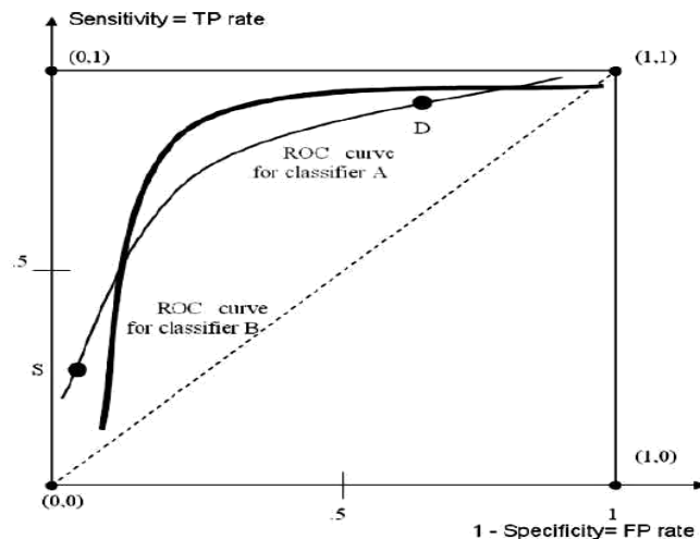
FIGURE.3.4: ROC Curve for two classifiers
