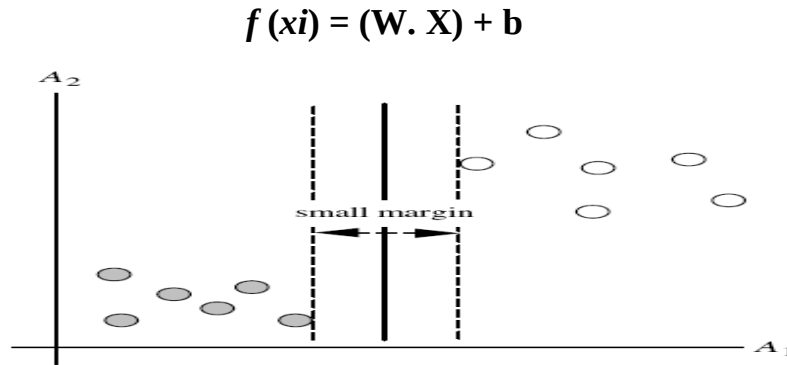
Figure 2.5: The 2-D training data are linearly separable.
