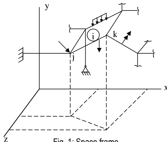
Fig. 1: Space frame
