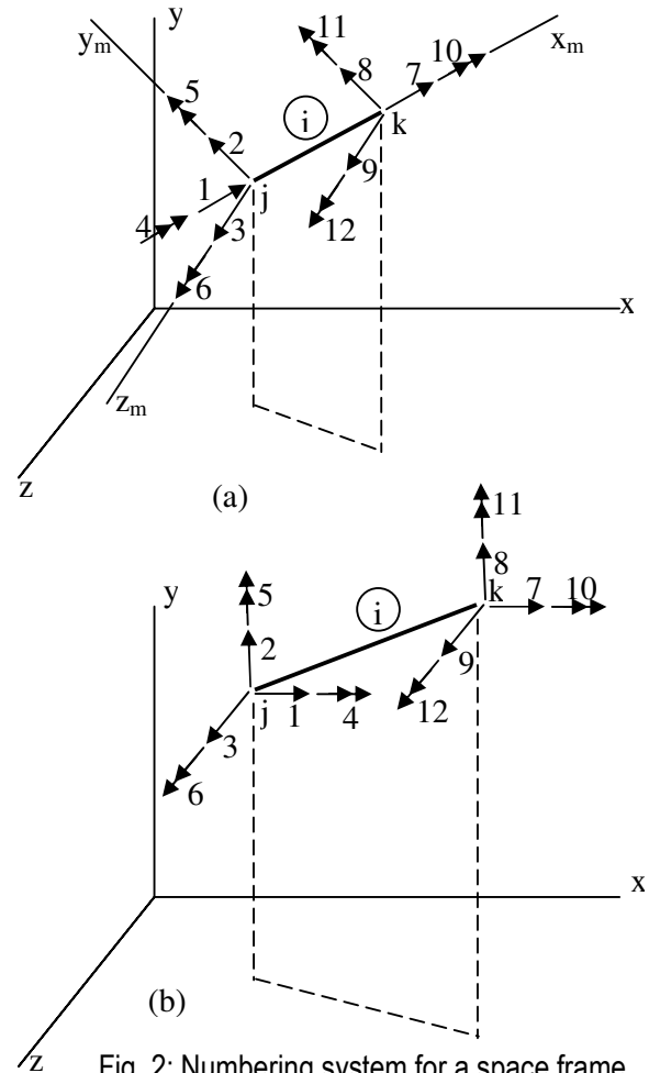
Fig. 2: Numbering system for a space frame
