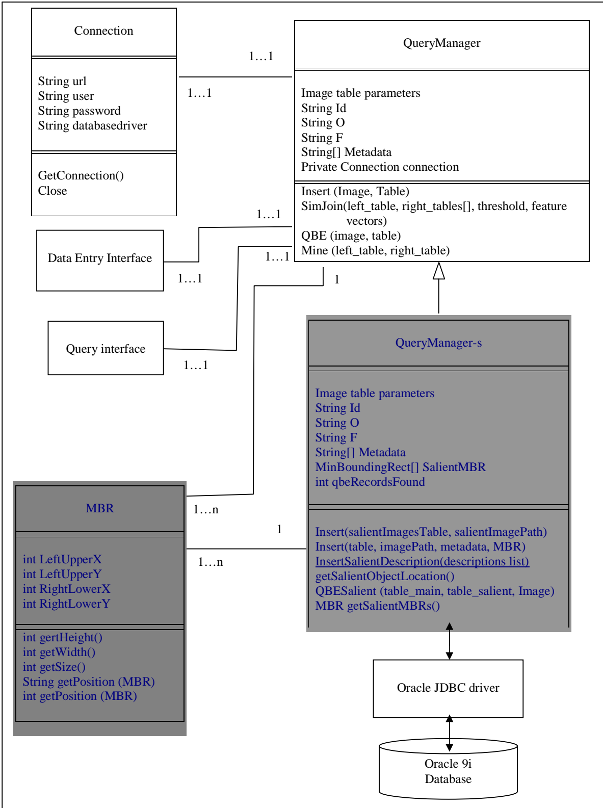
Figure 6-1 Structure of EMIMS-S
