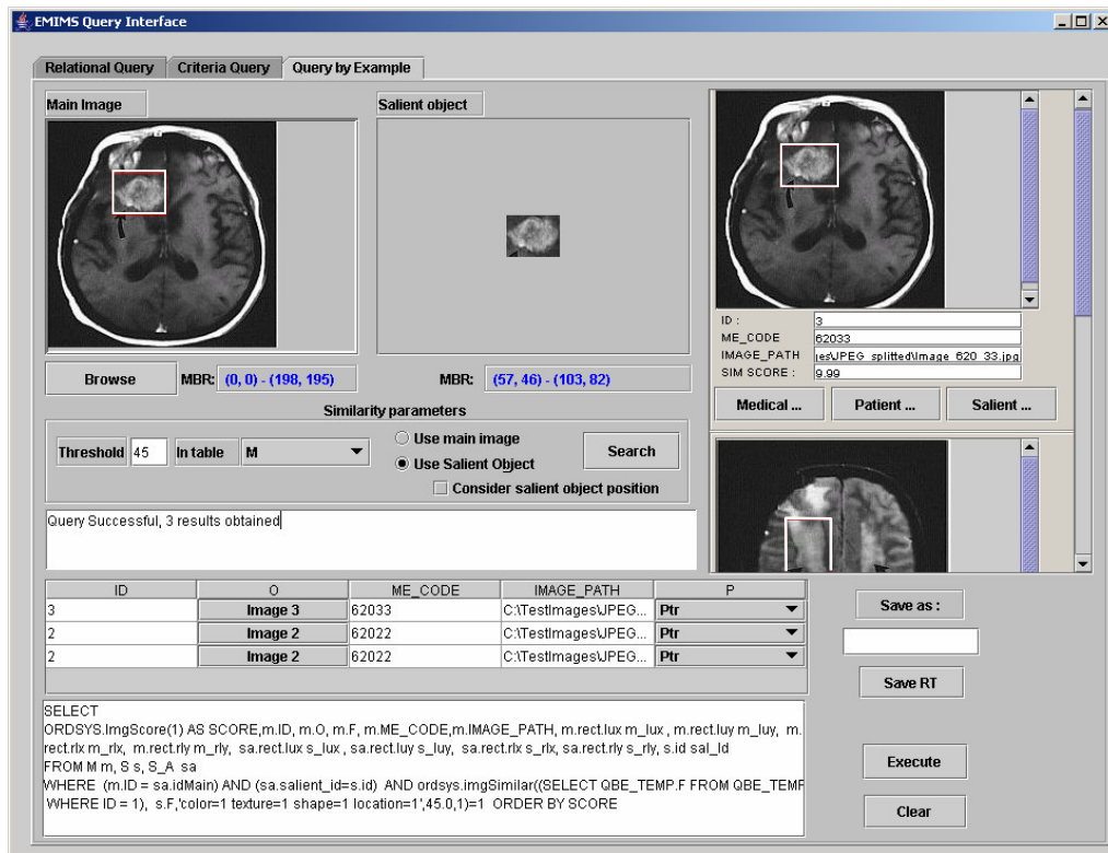
Figure 6-5 The query interface with salient-Object-based query integrated
