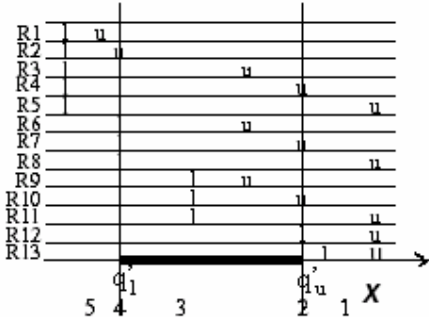
Figure 3-2 The 13 possible relations in 1D space [31]
