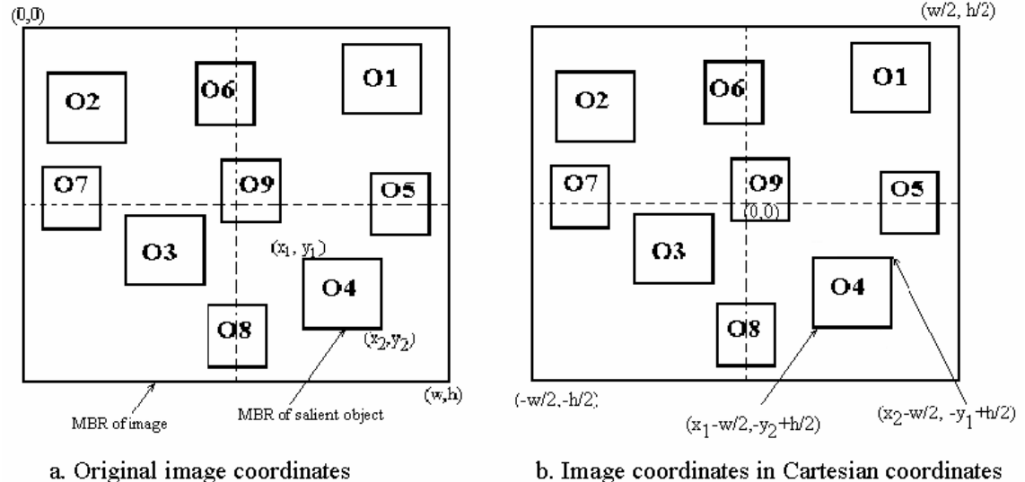
Figure 5-1 Salient objects positions within the main image
