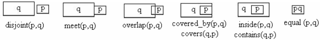
Figure 3-1 Topological Relations [31]
