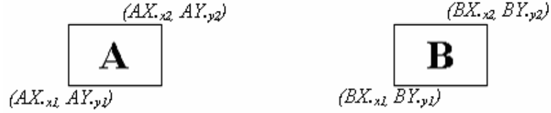
Figure 5-2 MBR representation of the projection of objects in two dimensional coordinate plane
