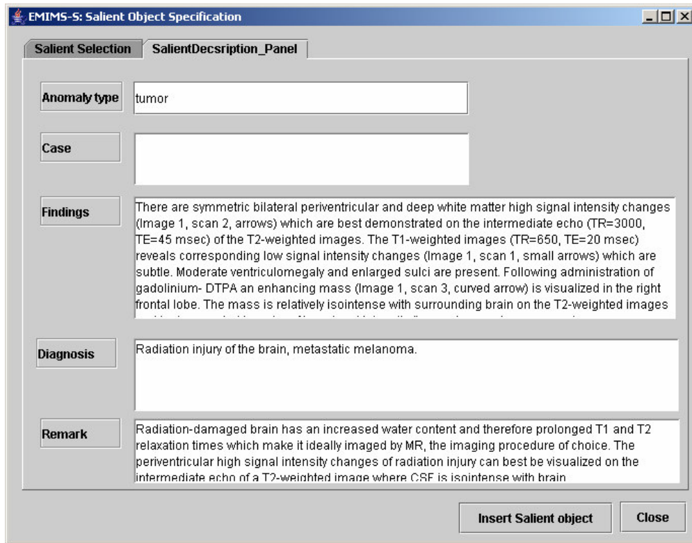
Figure 6-4 EMIMS-S Salient object metadata description interface
