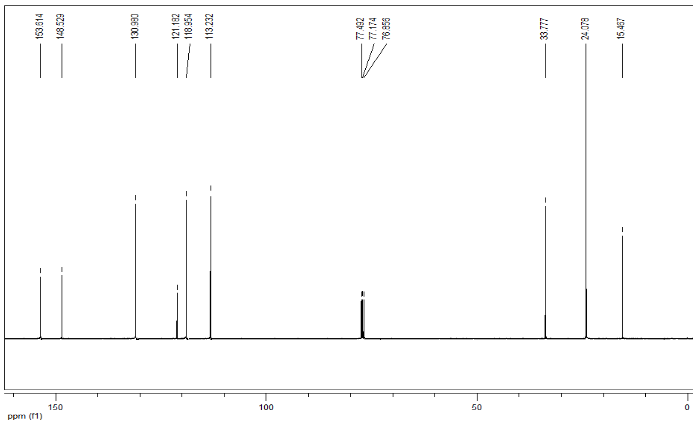
Appendix-7 ^{13}\text{C} NMR spectrum of pure carvacrol (400 MHz NMR)
