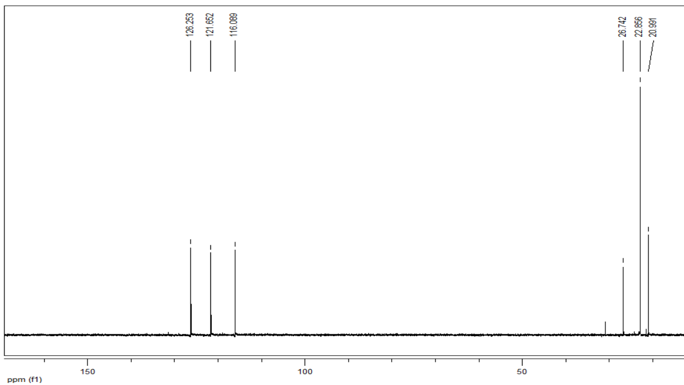
Appendix-2 DEPT-135 NMR spectrum of thymol isolated from Trachyspermum ammi EO
