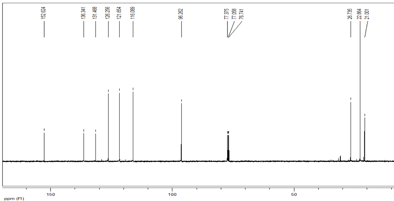
Appendix-1 ^{13}\text{C} NMR spectrum of thymol isolated from Trachyspermum ammi EO
