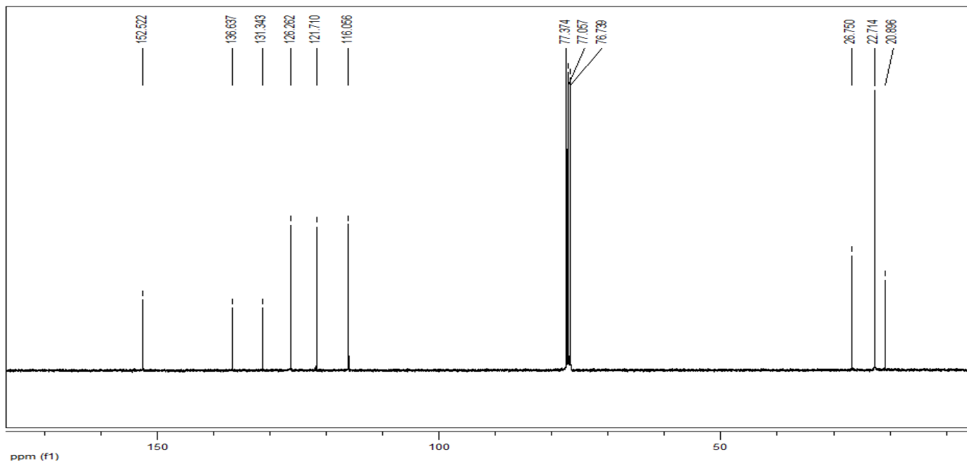
Appendix -5 ^{13}\text{C} NMR spectrum of pure thymol (400 MHz NMR)
