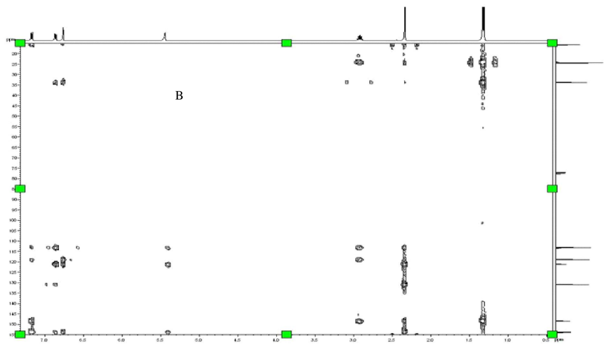
Fig. 12 HMBC NMR Spectrum of pure thymol (A) and pure carvacrol (B)
