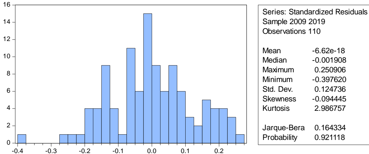
Figure 2 Normality Test
