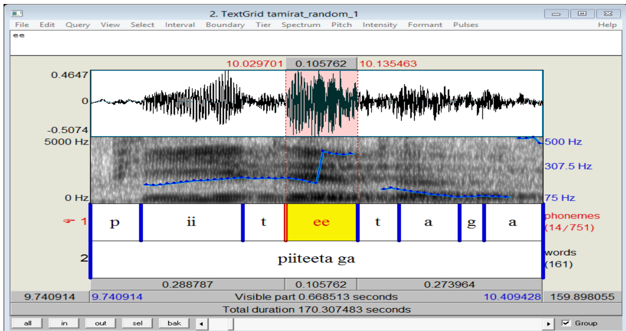
Figure 3.2: The sample extraction of the durational waveform of /e:/ in a tVVt frame (which is 106ms)
