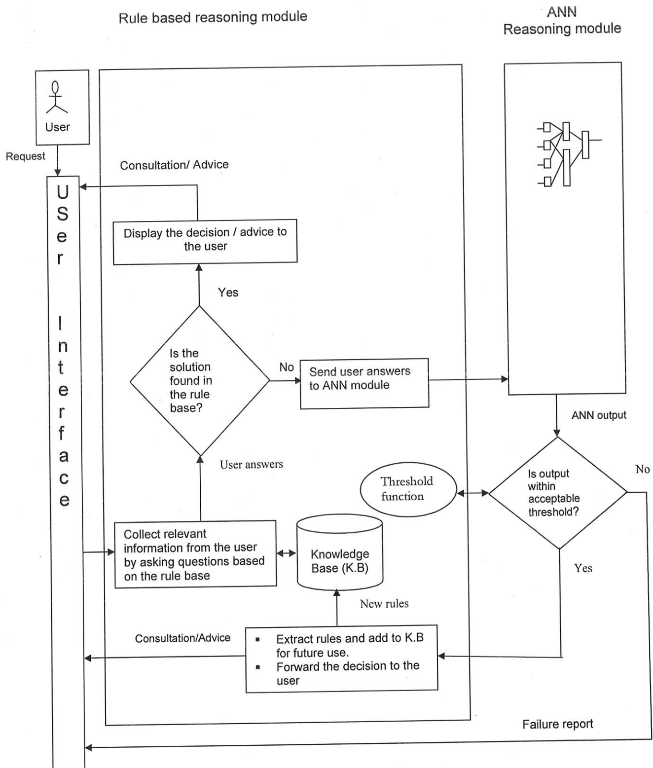
Fig 5.1 Model of the hybrid vegetable expert system
