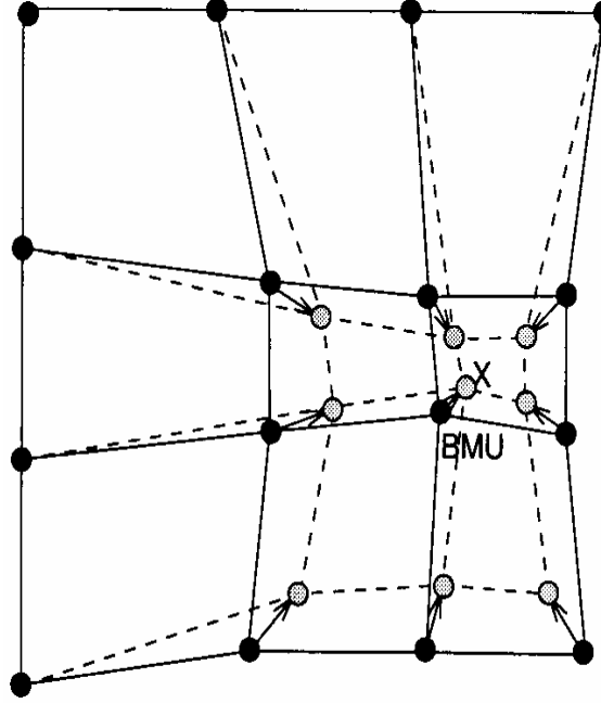
Figure 3.2. Updating the SOM and its neighbours towards the input sample marked with x . The solid and broken lines correspond to situation before and after updating (Vesanto et al. 2000).
