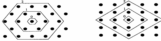
Figure 3.3. Neighbourhoods (0, 1 and 2) of the centre most unit: hexagonal grid on the left, rectangular on the right. The innermost polygon corresponds to 0, next to the 1- and the outermost to the 2-neighbourhood (Vesanto et al. 2000).
