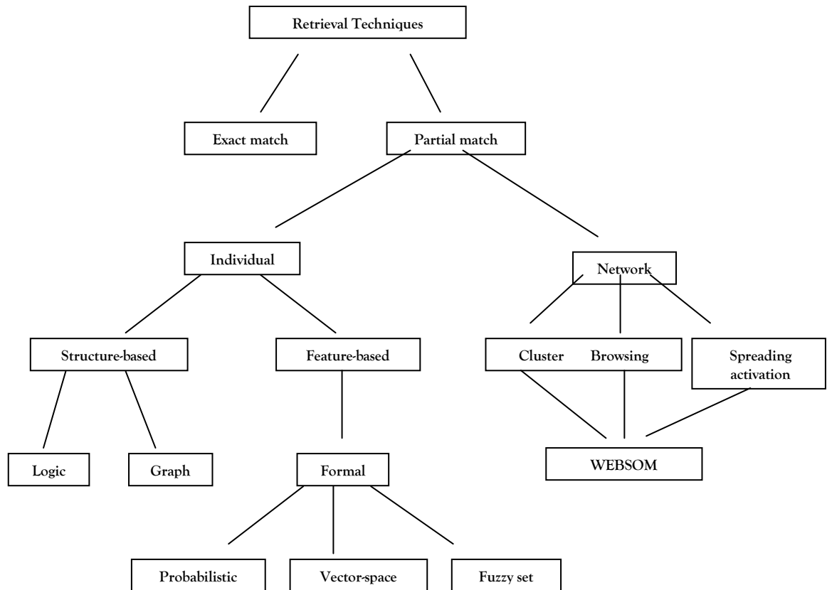
Figure 2.2. A classification of retrieval techniques (Adapted from Belkin and Croft 1987).
