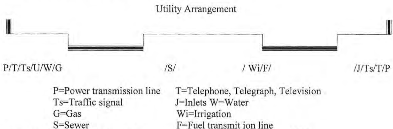
Figure 2.2, Figure showing the standard of utility arrangement
