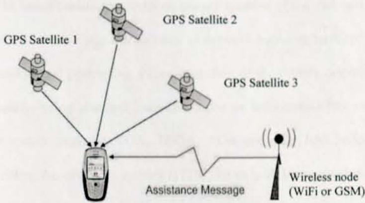
Figure 2-2: Principle of A-GPS
