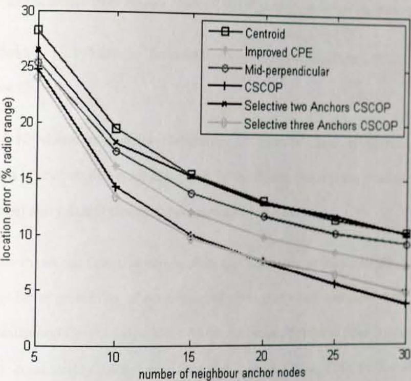
Figure 5-9: Average location error (% radio range) of Selective Anchor Nodes CSCOP in case of dense crowd
