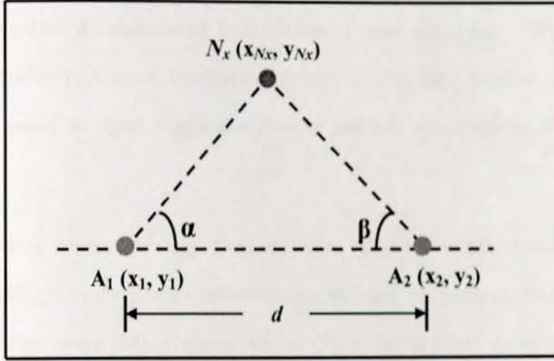
Figure 3-3: Angle of Arrival (AOA) Localization
