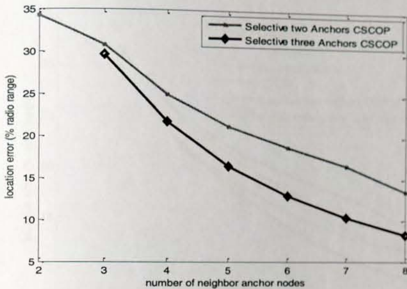
Figure 5-6: Average location error (% radio range) of Selective two and Selective three CSCOP in case of sparse crowd
