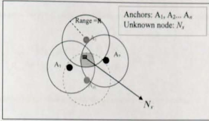
Figure 3-6: Centroid algorithm geo-localization
