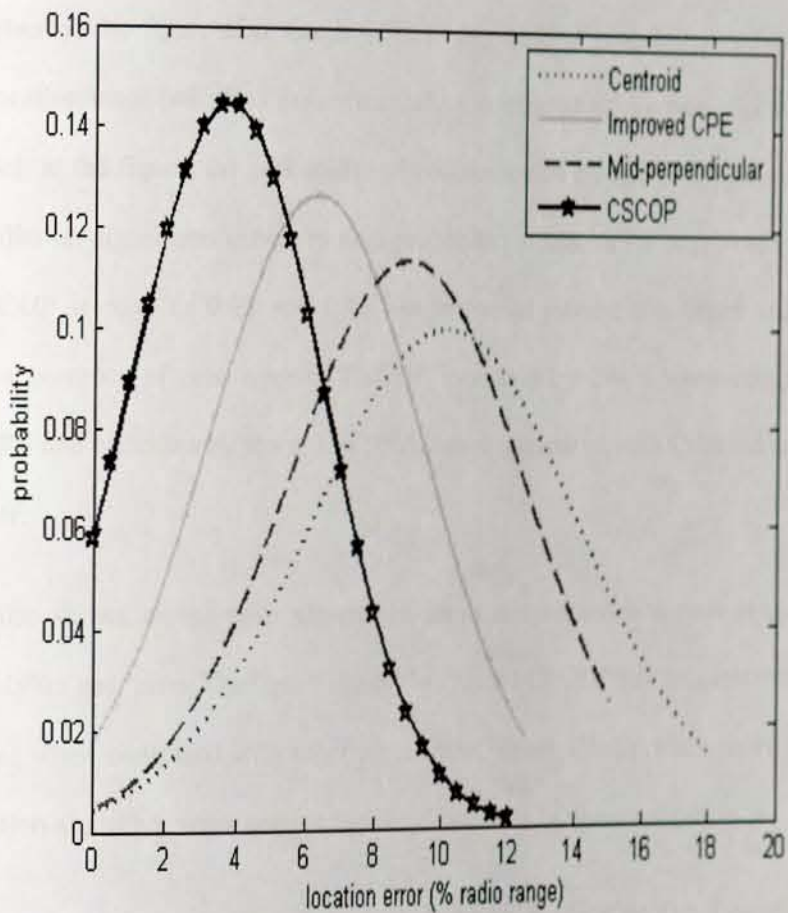
Figure 5-5: Probability distribution of location error of CSCOP in case of dense crowd (30 neighbour anchor nodes)
