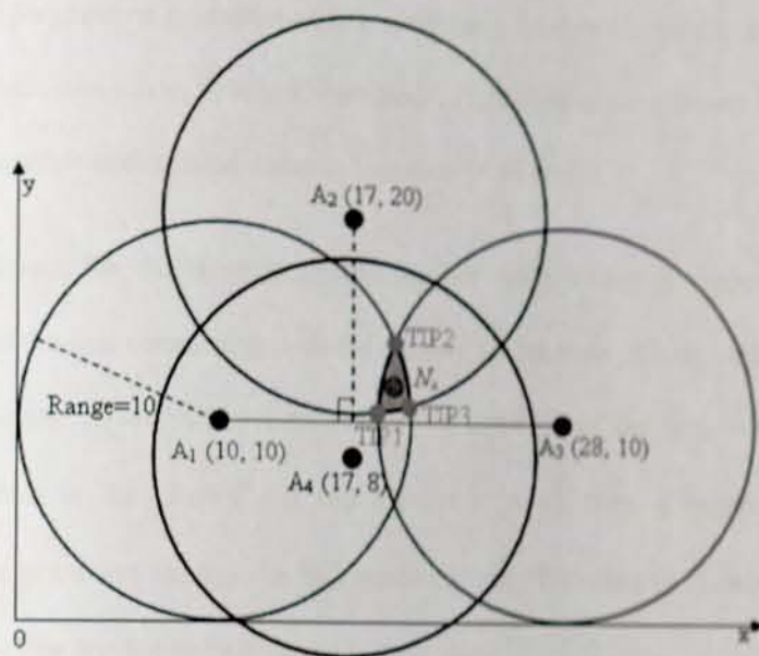
Figure 4-8: Principle of Selective three Anchor Nodes CSCOP Algorithm
