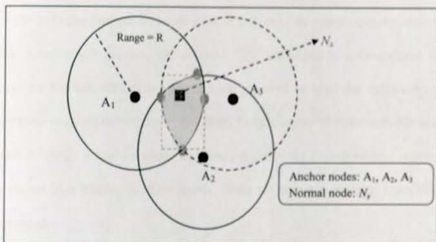
Figure 3-8: Example of CPE algorithm
