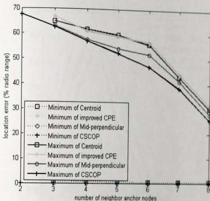
Figure 5-2: Maximum and minimum location error in (% of radio range) of CSCOP in sparse crowd
