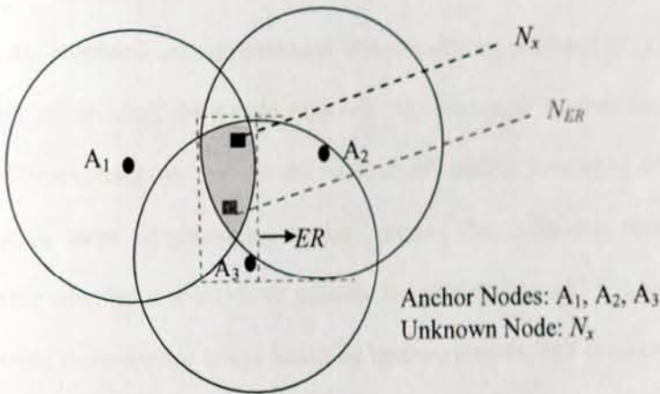
Figure 3-10: Improved CPE Algorithm
