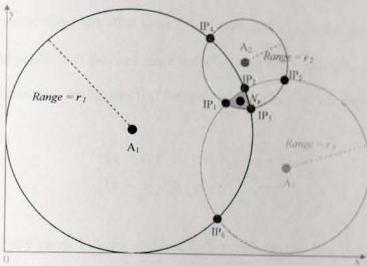
Figure 4-10: Finding Intersection Points (IPs)
