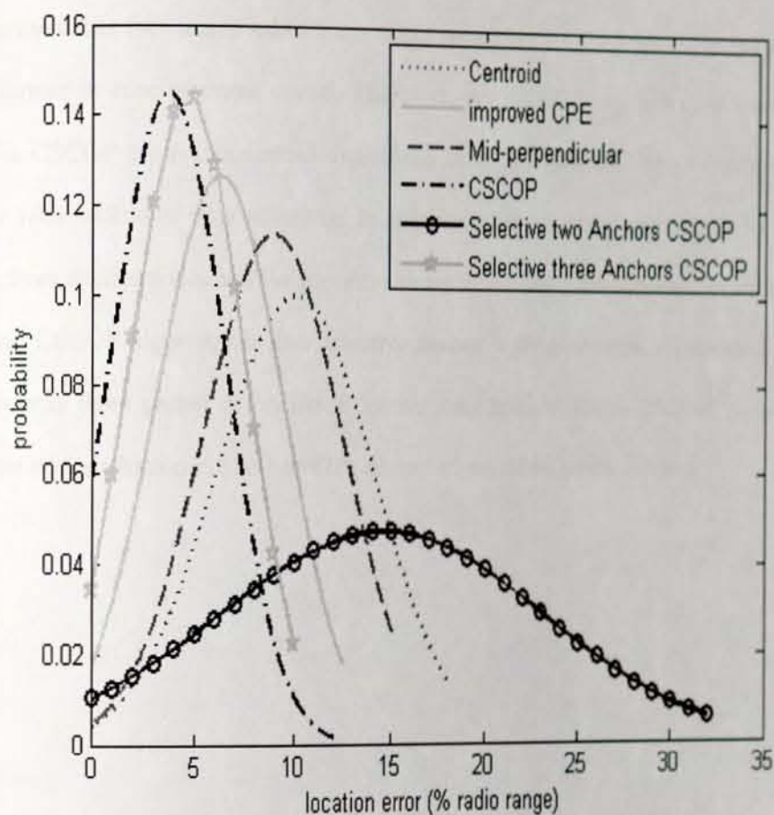
Figure 5-10: Probability distribution of location error of Selective CSCOP in case of dense crowd (30 neighbour anchor nodes)
