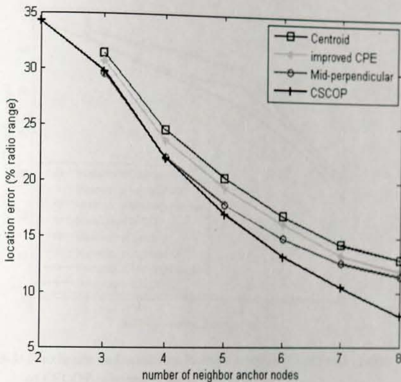
Figure 5-1: Average location error (% radio range) of CSCOP in sparse crowd
