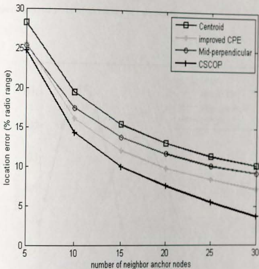
Figure 5-4: Average location error (% radio range) of CSCOP in case of dense crowd
