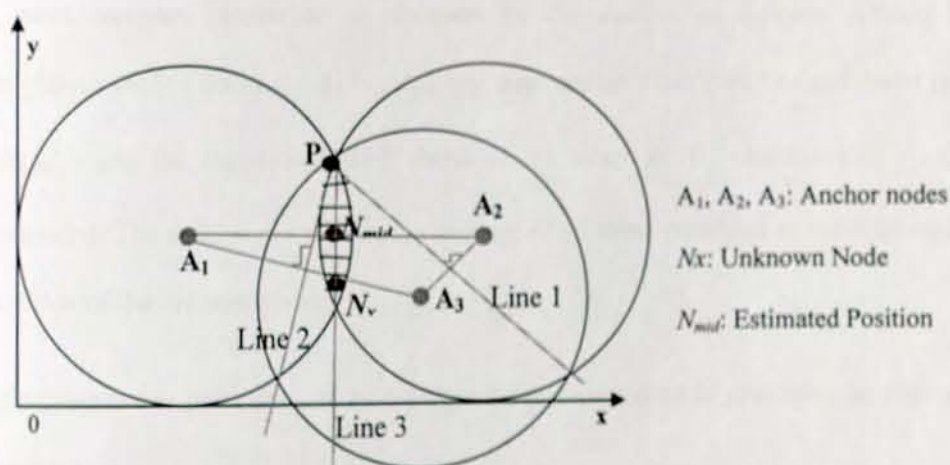
Figure 3-17: Mid-perpendicular algorithm when an Obtuse Angled Triangle (with 3 neighbour anchor nodes)
