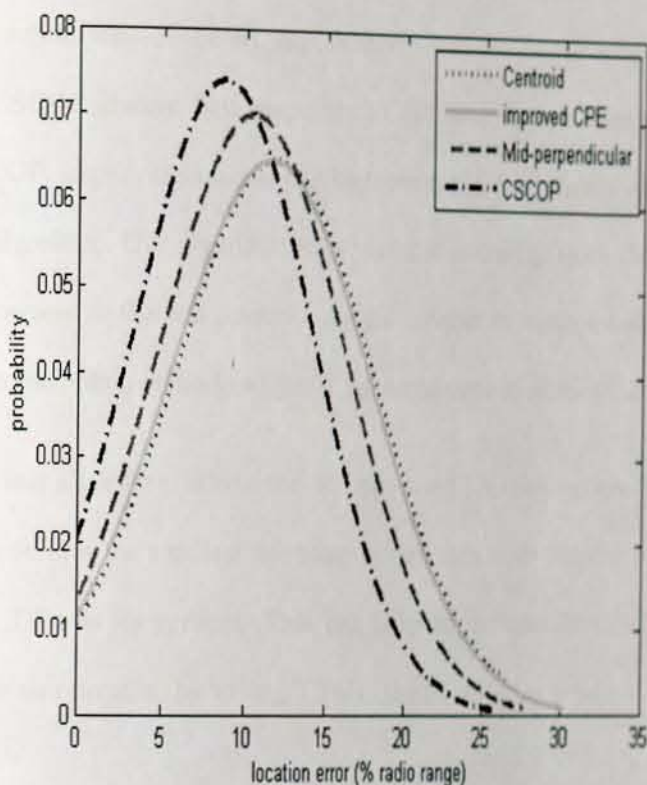
Figure 5-3: Probability distribution of CSCOP location error in sparse crowd (8 neighbour anchor nodes)
