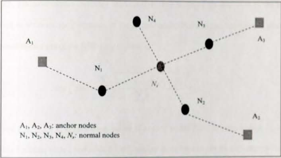
Figure 3-19: Example of network topology for DV-hop algorithm
