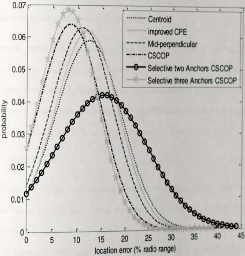
Figure 5-8: Probability distribution of location error of Selective CSCOP in case of sparse crowd (8 neighbour anchor nodes)
