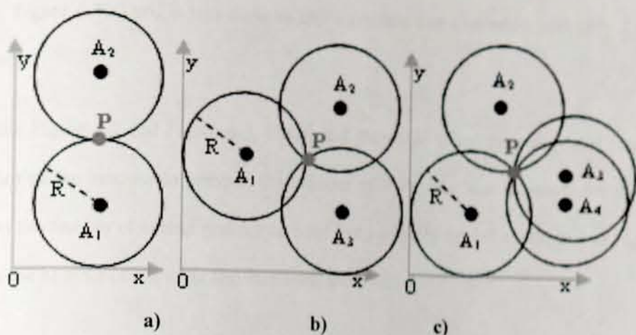
Figure 4-2: Senario-1, SCOP with one TIP regardless of increase in number of anchor nodes
