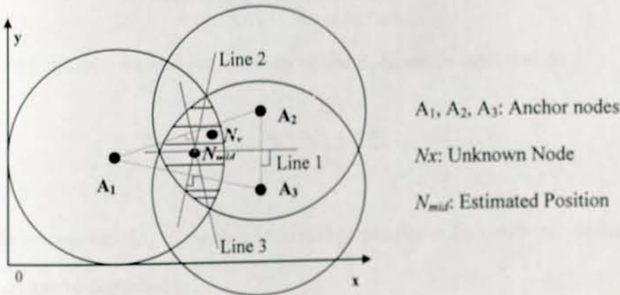
Figure 3-15: Mid-Perpendicular when an Acute Triangle (with 3 neighbour anchor nodes)
