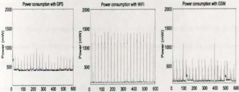
Figure 2-3: Energy consumption of GPS, WiFi and GSM for position fixes every 30 seconds
