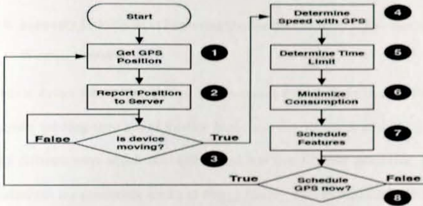
Figure 2-8: System logic of EnTracked
