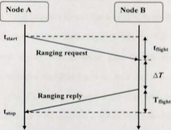
Figure 3-5: Two-Way Ranging
