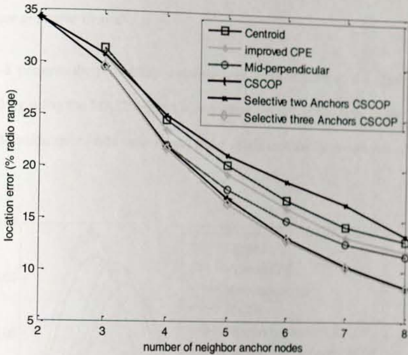
Figure 5-7: Average location error (% radio range) of Selective CSCOP in case of sparse crowd
