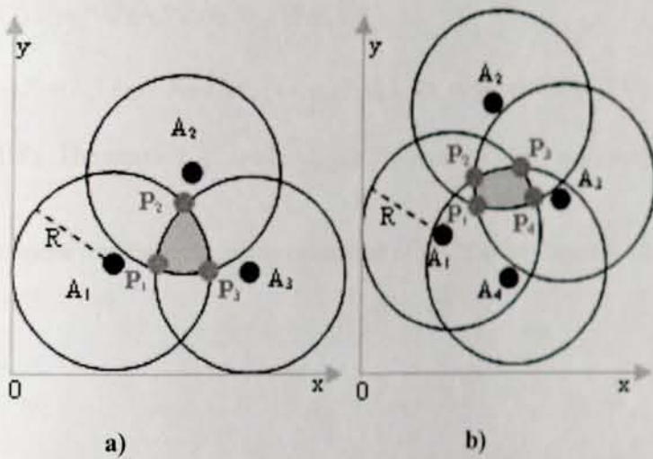
Figure 4-4: Scenario-3, SCOP with more than 2 TIPs
