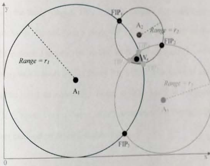
Figure 4-11: Identifying True Intersection Points (TIPs) from False Intersection Points (FIPs)
