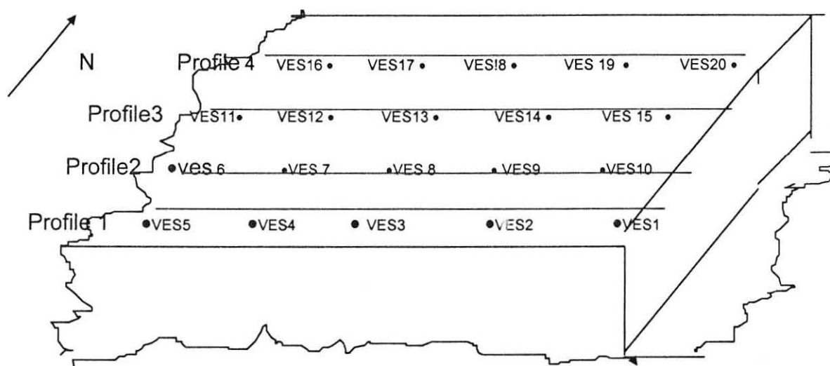
Fig.(12) schematic diagram showing sounding stations and profiles
