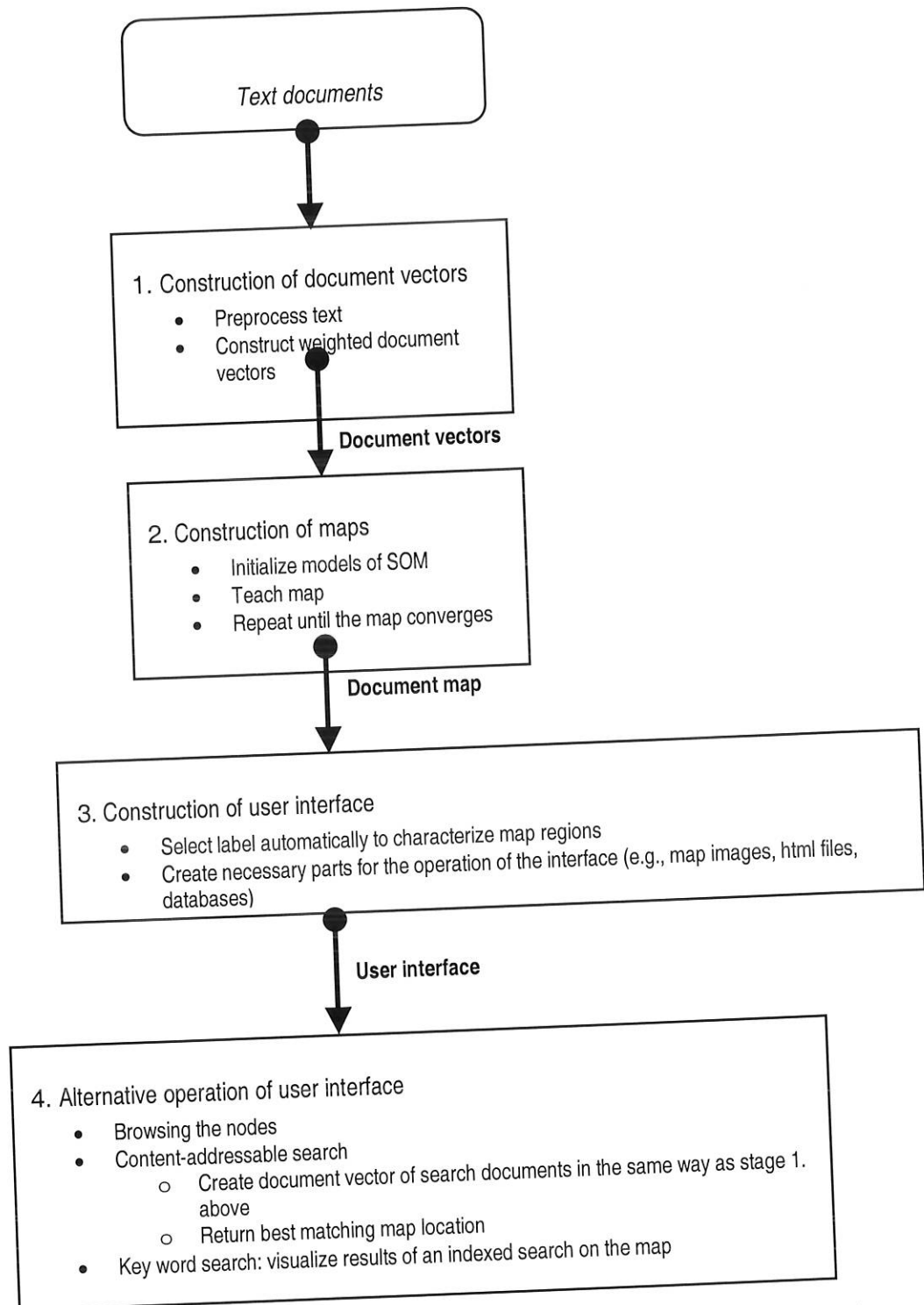
Figure 2.1 The basic architecture of the WEBSOM method (Honkela et al., 1996; Kohonen, 2000).
