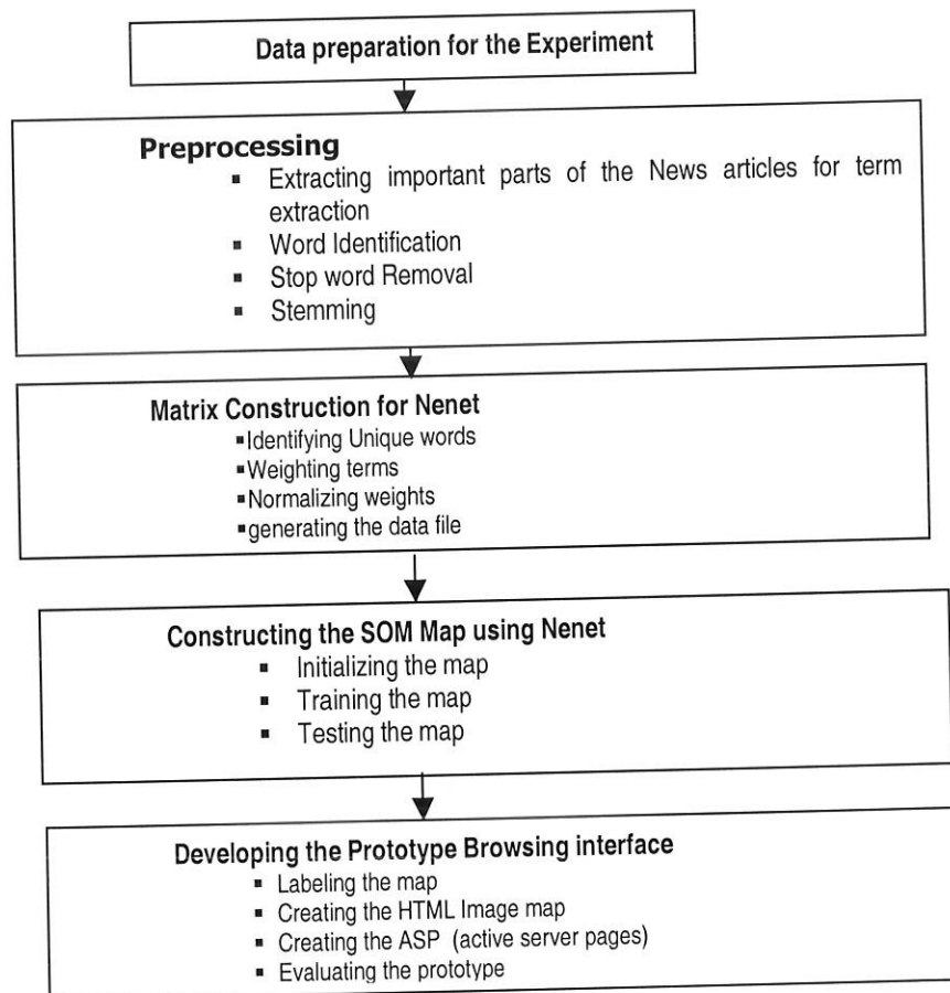
Figure 3.1 Self-organized Map developments.
