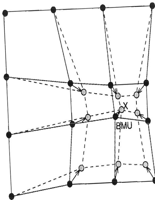
Figure 2.4. Updating the SOM and its neighbours towards the input sample marked with x.. The solid and broken lines correspond to situation before and after updating (Vesanto et al. 2000)
