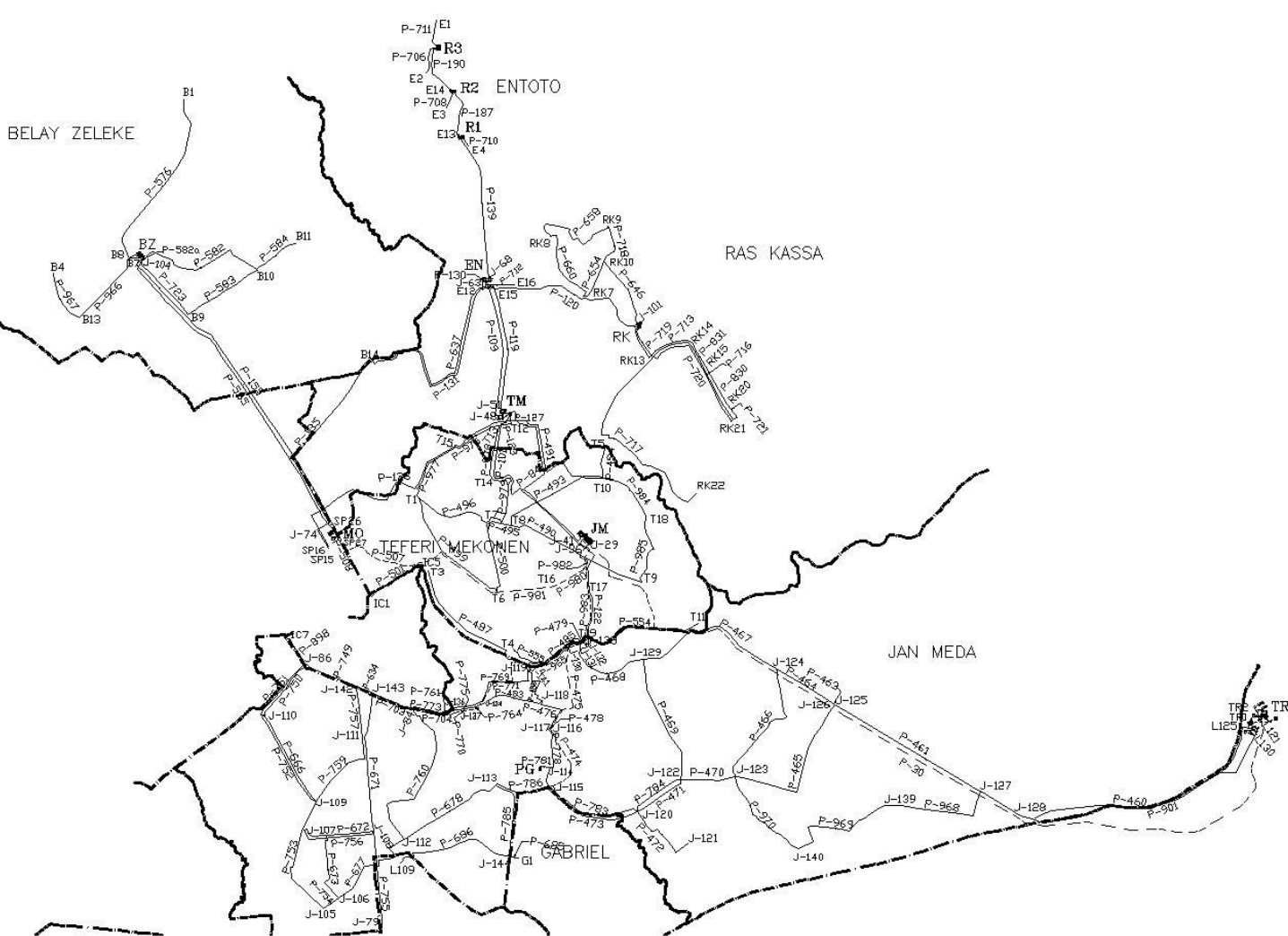
Figure (4.2): Layout of Existing water system of the Study area
