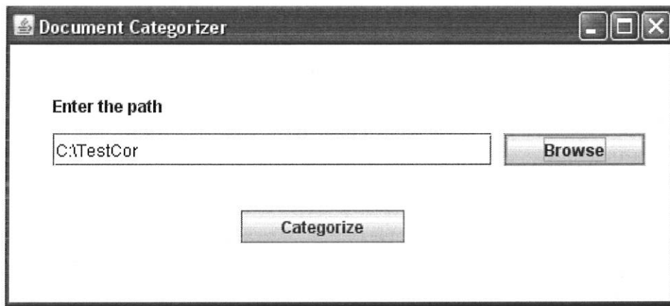
Figure 4.13: User Interface
