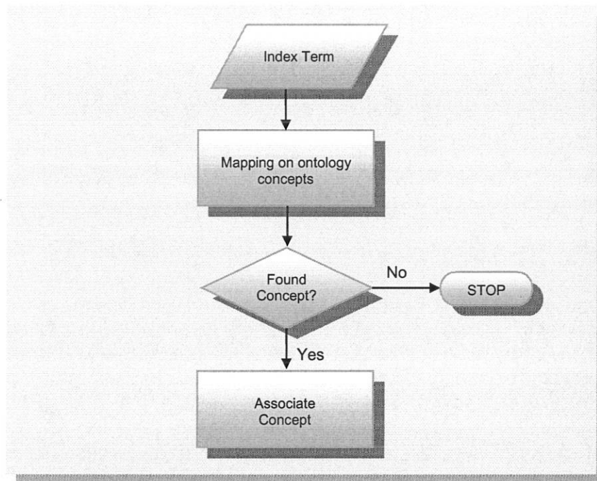
Figure 4.16: The flowchart of the mapping between terms and the News ontology concepts
