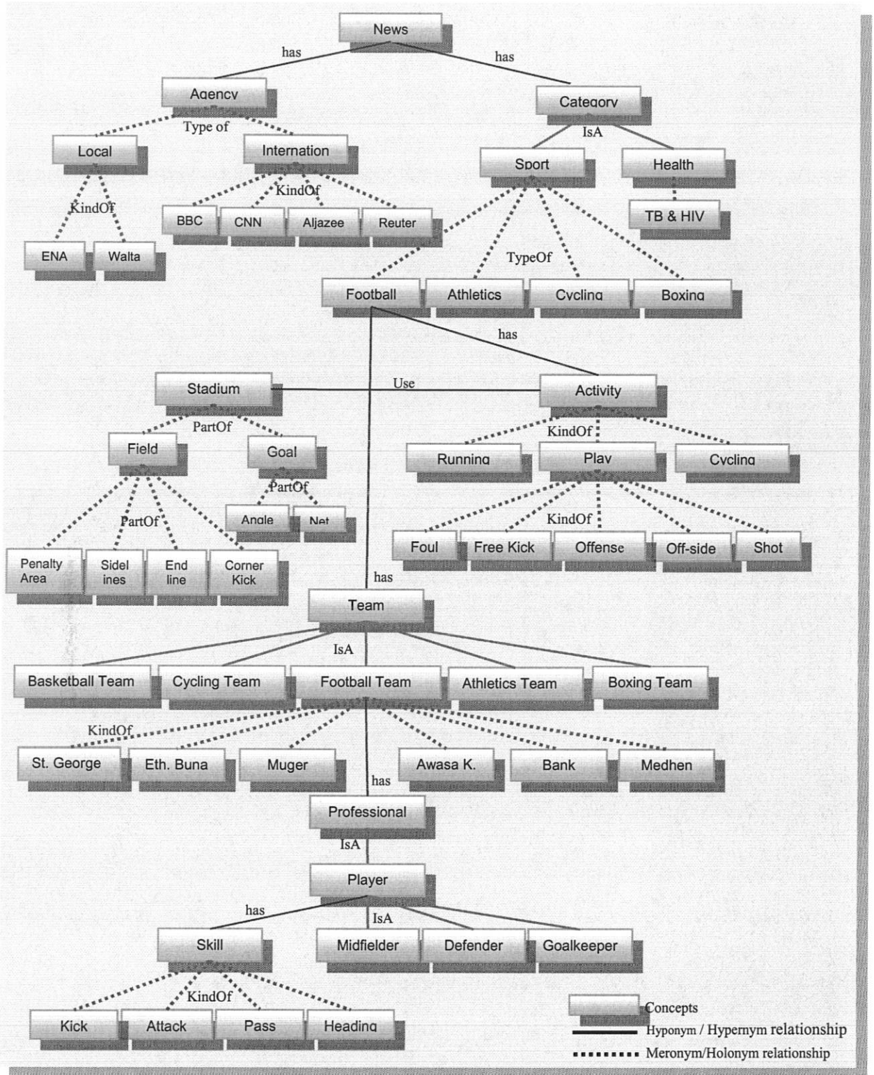
Figure 4.6: Concepts and Relations in the News ontology
