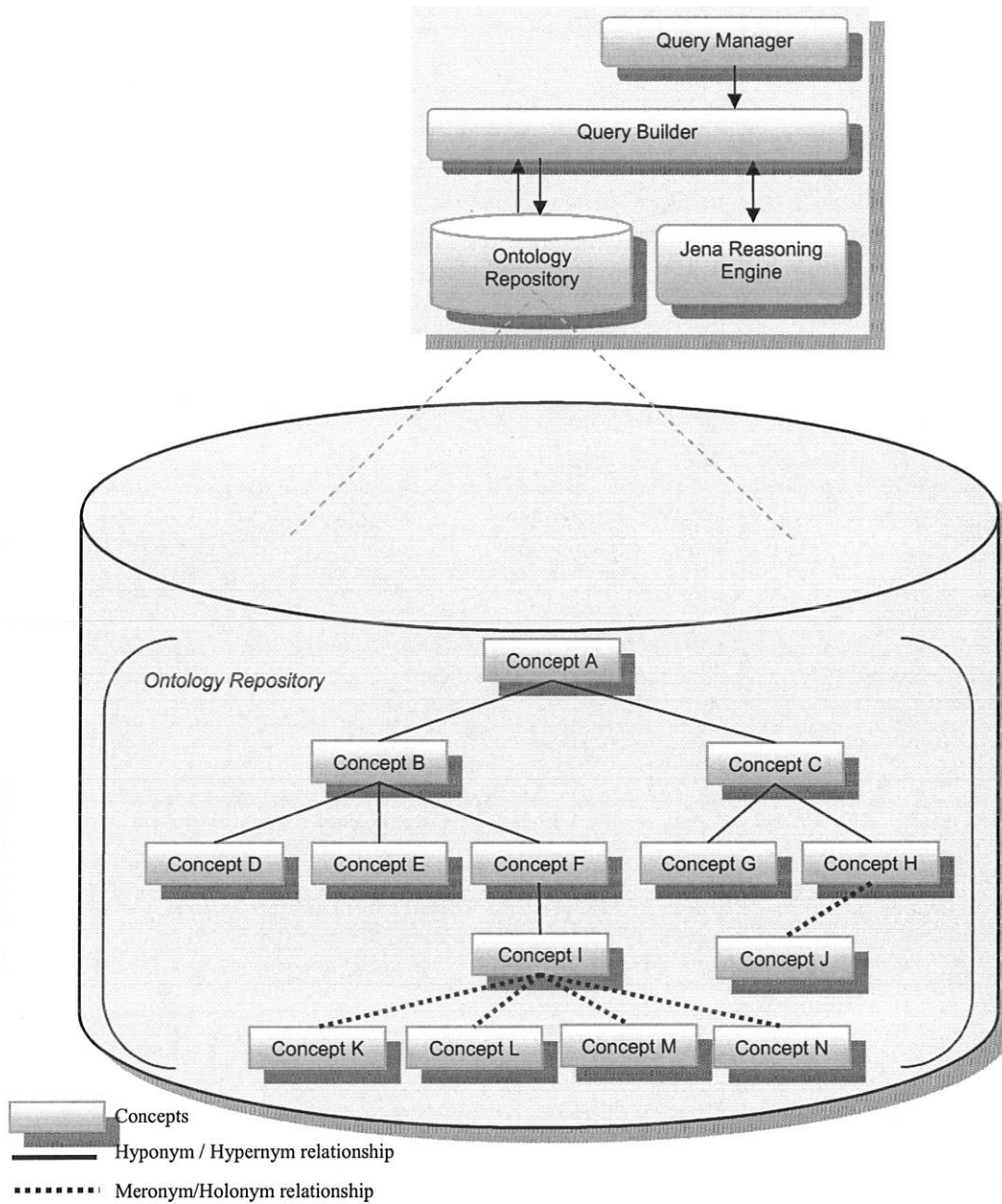
Figure 4.3: The architecture of the ontology
