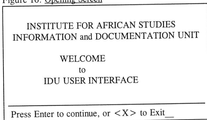
Figure 16: Opening Screen
