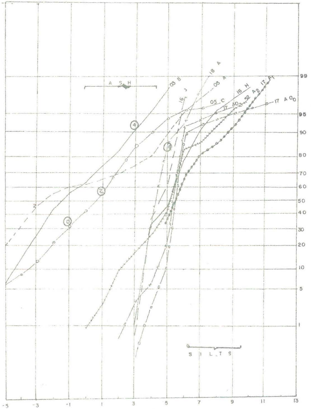
Fig. 15 CUMULATIVE CURVES OF GRAIN-SIZE DISTRIBUTIONS FOR ASH & SILTS OF THE UPPER SEQUENCE. — CIRCLED NUMBERS INDICATE VALUES OF DIAMETERS.
