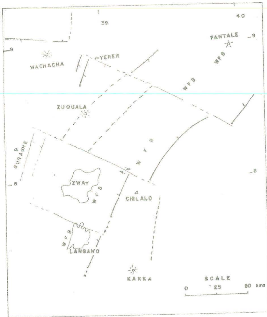
FIG. 2 SCHEMATIC TECTONIC MAP OF THE RIFT SHOWING THE WONJI FAULT BELT (WFB) AFTER P.A. MOHR (1967).
