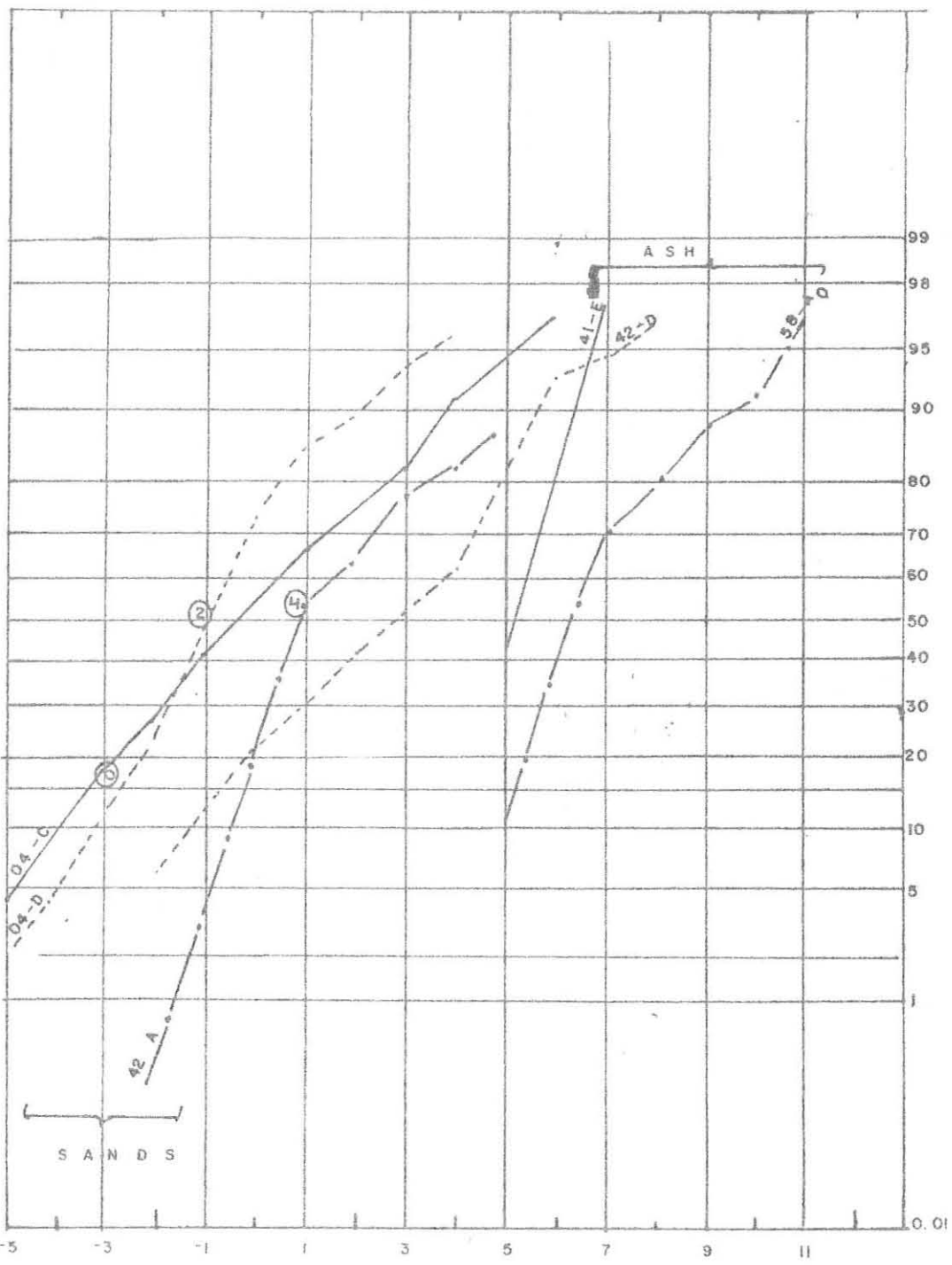
Fig. 9 CUMULATIVE CURVES OF GRAIN-SIZE DISTRIBUTIONS FOR SANDS & ASH SAMPLES OF LOWER SEQUENCE. - CIRCLED NUMBERS INDICATE VALUES OF DIAMETERS.
