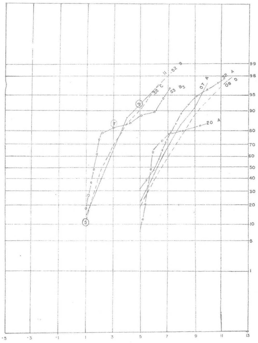
Fig. 16 CUMULATIVE CURVES OF GRAIN-SIZE DISTRIBUTIONS FOR DIATOMITES OF THE UPPER SEQUENCE.
