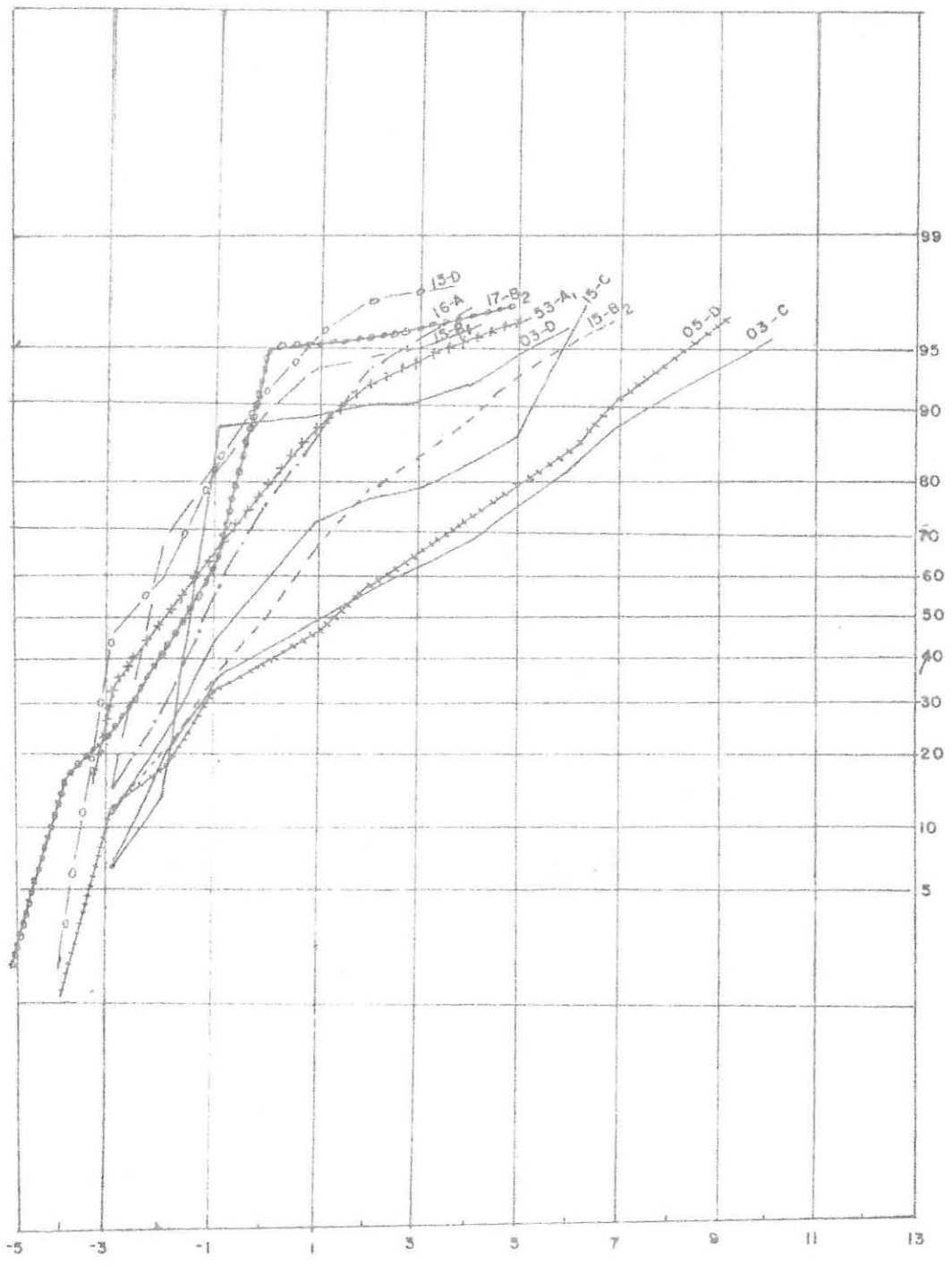
Fig. 15 CUMULATIVE CURVES OF GRAIN-SIZE DISTRIBUTIONS FOR GRAVELS OF THE UPPER SEQUENCE
