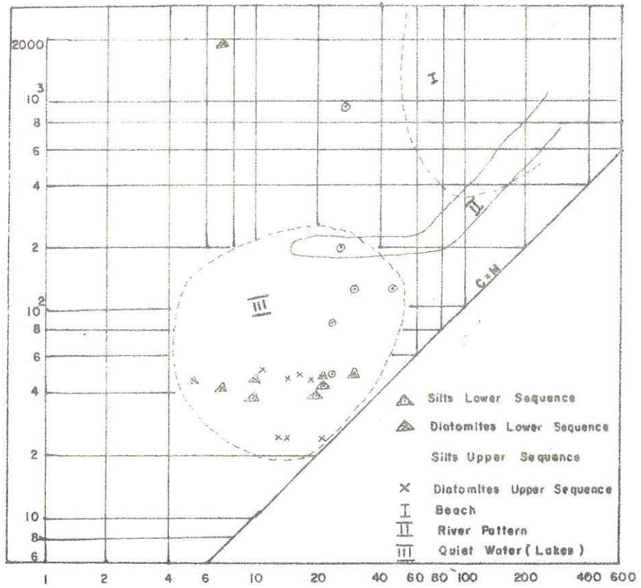
Fig. 20 CM DIAGRAM OF ADAMI TULU SEDIMENTS
