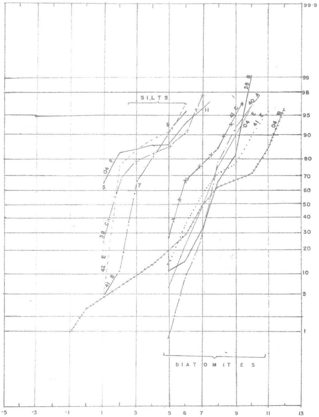
Fig. 10 CUMULATIVE CURVES OF GRAIN-SIZE DISTRIBUTIONS FOR SILTS AND DIATOMITES OF LOWER SEQUENCE.
