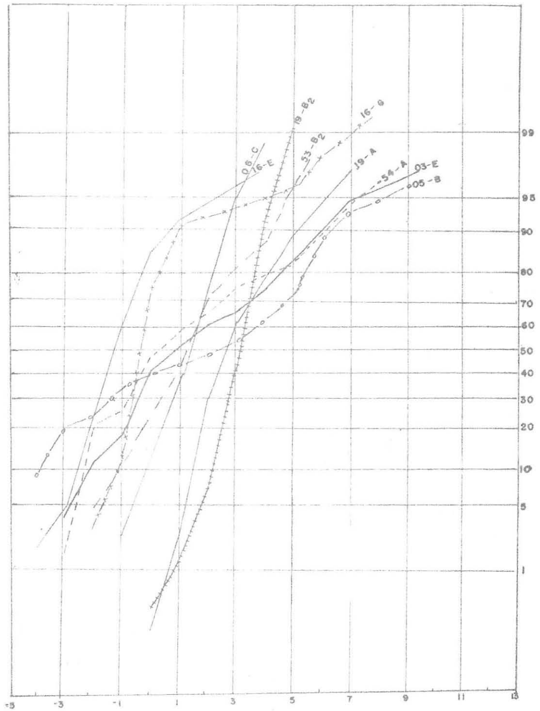
Fig. 144 CUMULATIVE CURVES OF GRAIN-SIZE DISTRIBUTIONS FOR THE SANDS OF THE UPPER SEQUENCE.
