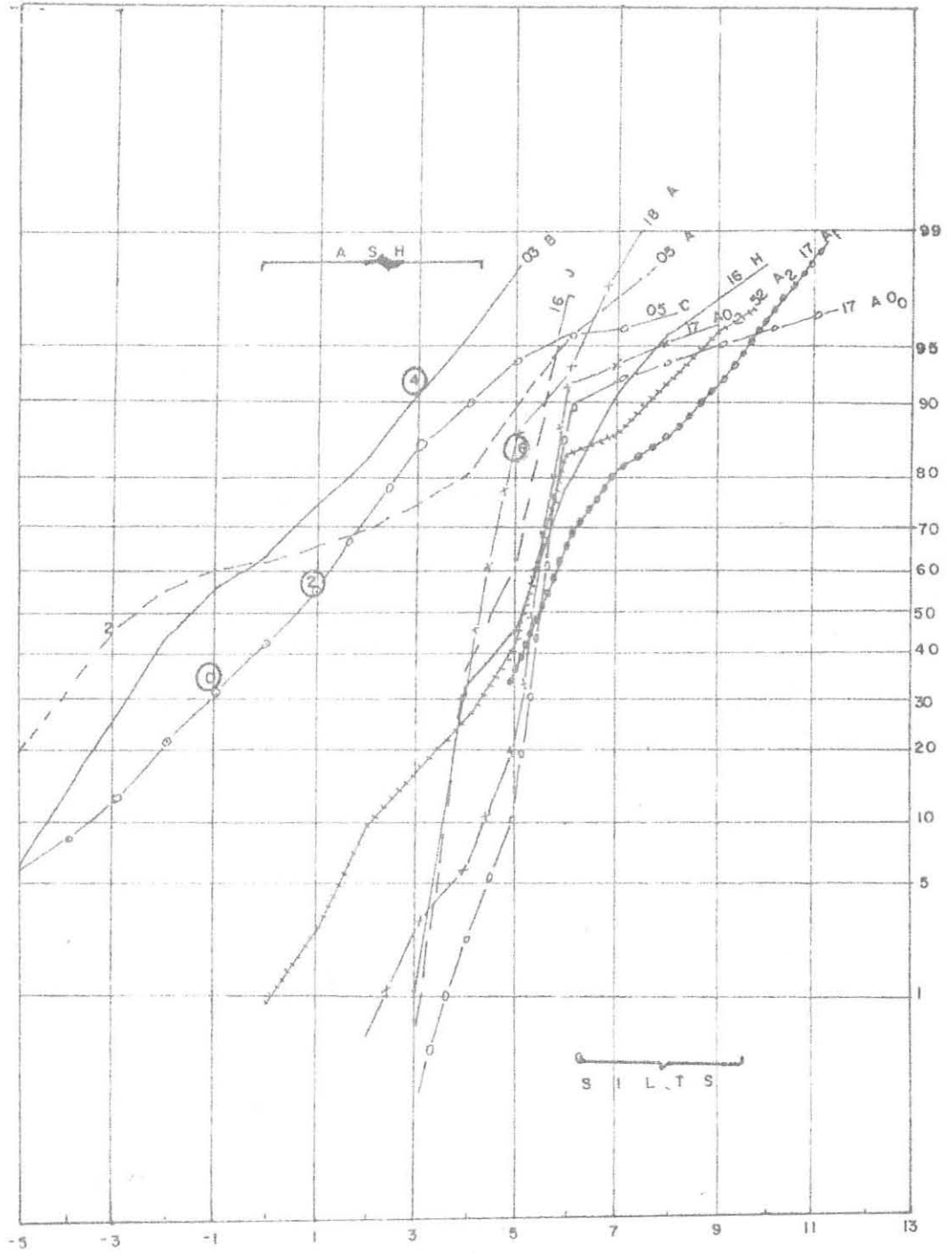
Fig. 15 CUMULATIVE CURVES OF GRAIN-SIZE DISTRIBUTIONS FOR ASH & SILTS OF THE UPPER SEQUENCE.
