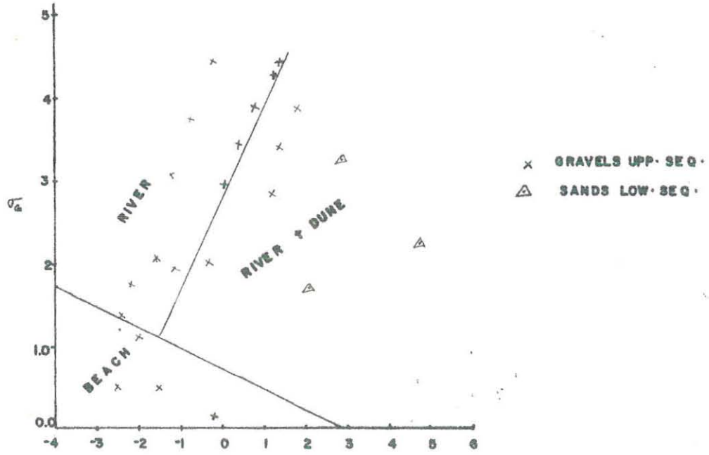
Fig. 15 PLOT OF STANDARD DEVIATION ( \sigma ) AGAINST MEAN ( m ).
