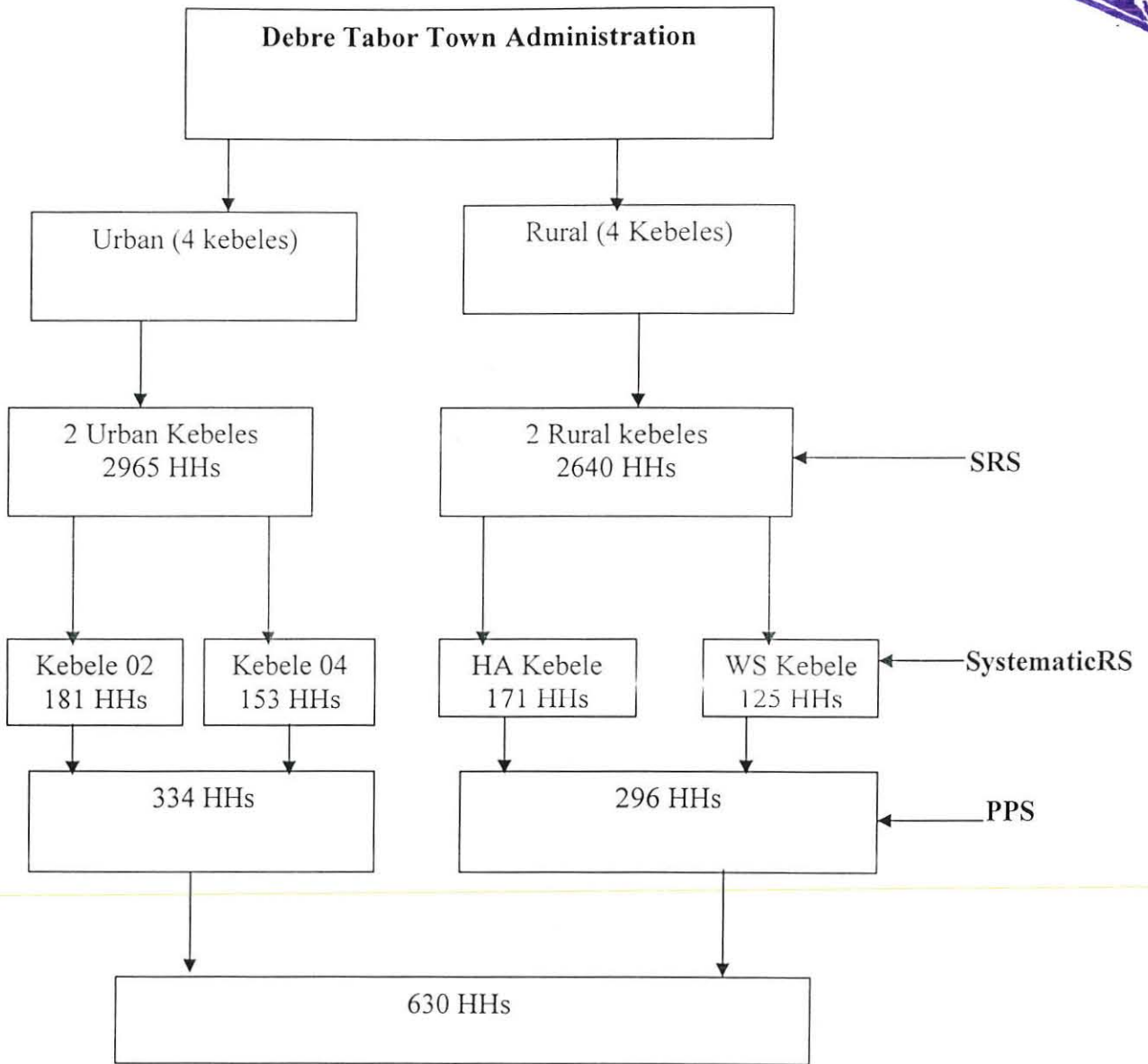
Figure 2: Sampling Procedure
