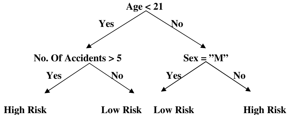
Figure 4.4: A simple Decision tree
