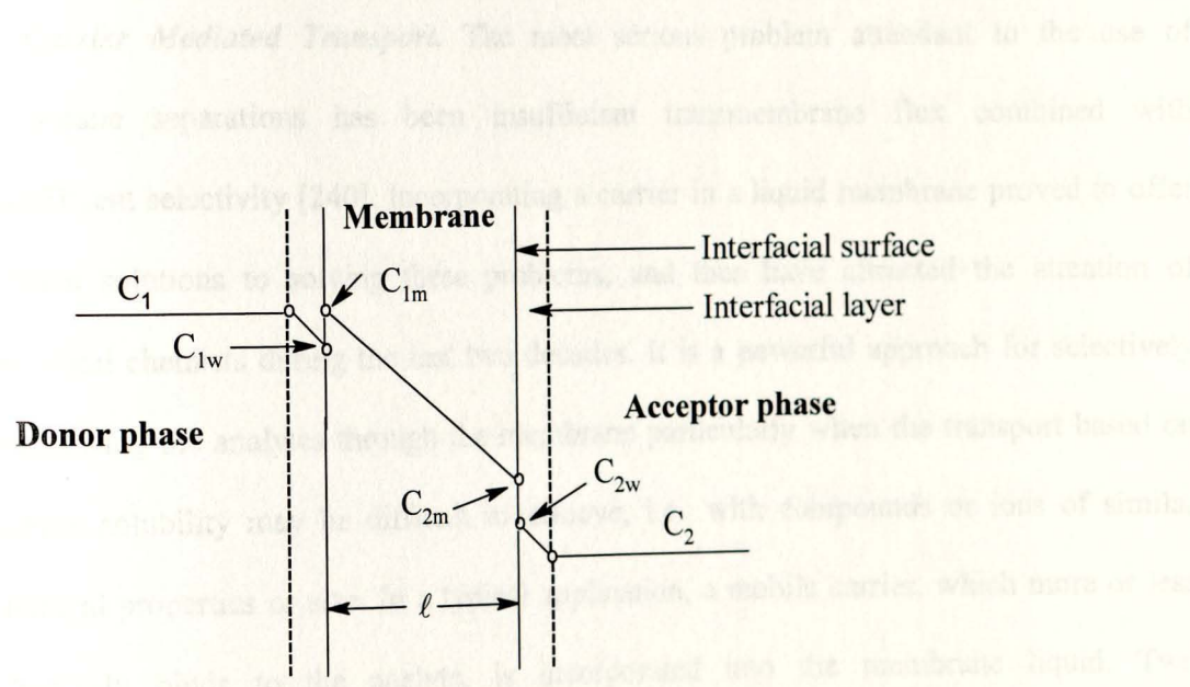
Fig. 1.8 A schematic representation of an idealized concentration profile of the analyte through the liquid membrane.
