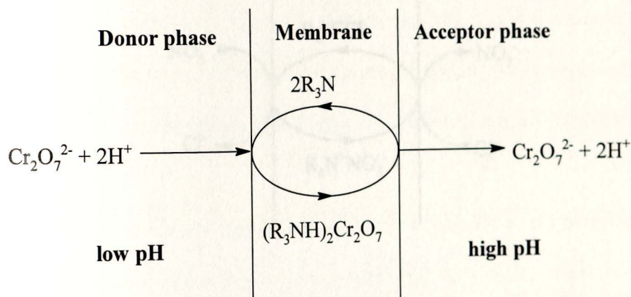
Fig. 1.9 Selective extraction of dichromate ion by coupled co-transport mechanism through the liquid membrane.
