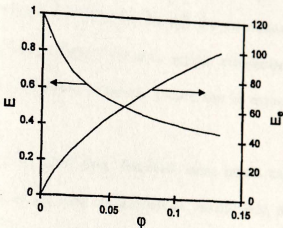
Fig. 1.12 Extraction efficiency, E , and enrichment factor, E_e , (arbitrary units) as a function of reduced flow parameter, \phi [85].
