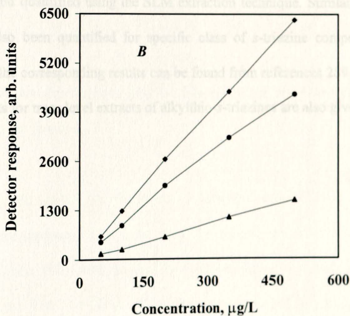
Fig. 3.11 Calibration graph for extraction of varied concentration of the sample mixture at donor flow rate of 1.0 mL/min. (A) di- n -hexylether, symbols: ♦ - atrazine, ● - prometone, and ▲ - propazine, and (B) n -undecane membrane solvents; symbols: ♦ - prometone, ● - terbutryn, and ▲ - propazine.
