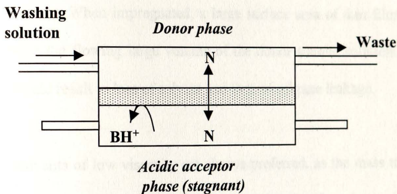
Fig. 1.11 Schematic representation of the SLM extraction of basic samples: (A) - extraction step, in the presence of acidic and neutral substances; and (B) - washing after extraction.
