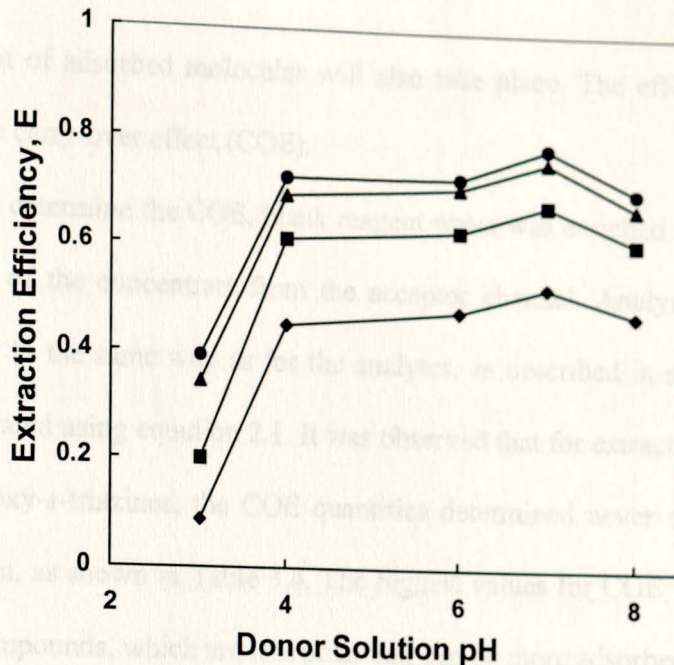
Fig. 3.3 Extraction efficiency, E , versus the donor pH for methoxy- s -triazine herbicides at the donor flow rate of 1.0 mL/min, 100% di- n -hexylether and 25 \mu L injection of the extracts. Symbols: (◆) -simetone; (■) - atratone; (▲) - secbumetone; and (●) - terbumetone.
