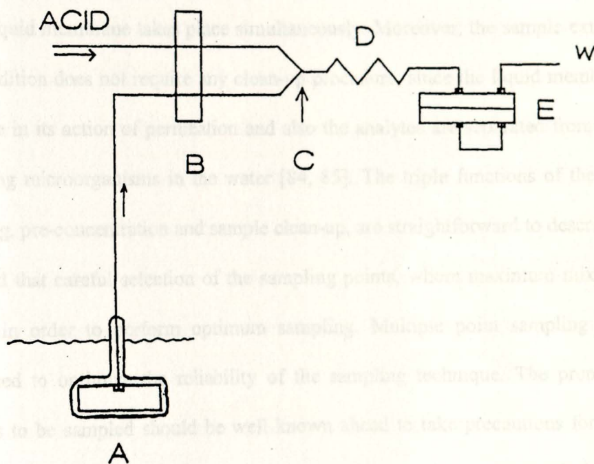
Fig. 1.5 Set-up for integrated field sampling: A - sampling compartment; B - peristaltic pump; C - confluence point of the sample stream; D - mixing coil; E - membrane separator; and W - waste [82].
