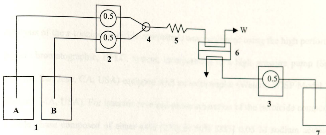
Fig. 2.3 Set-up of the flow system for liquid membrane extraction: (1) containers for sample solution (A) and donor buffer (B); (2) and (3) peristaltic pumps for the donor and acceptor channels, respectively; (4) PTFE tee connection; (5) mixing coil; (6) membrane extraction unit; (7) container for acidic acceptor solution; and (W) waste.
