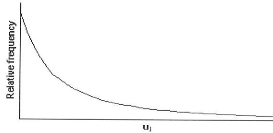
Figure 4 Exponential Distribution
