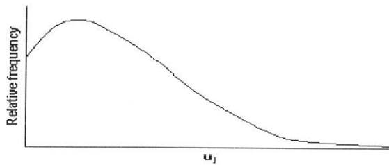
Figure 3 Truncated normal
