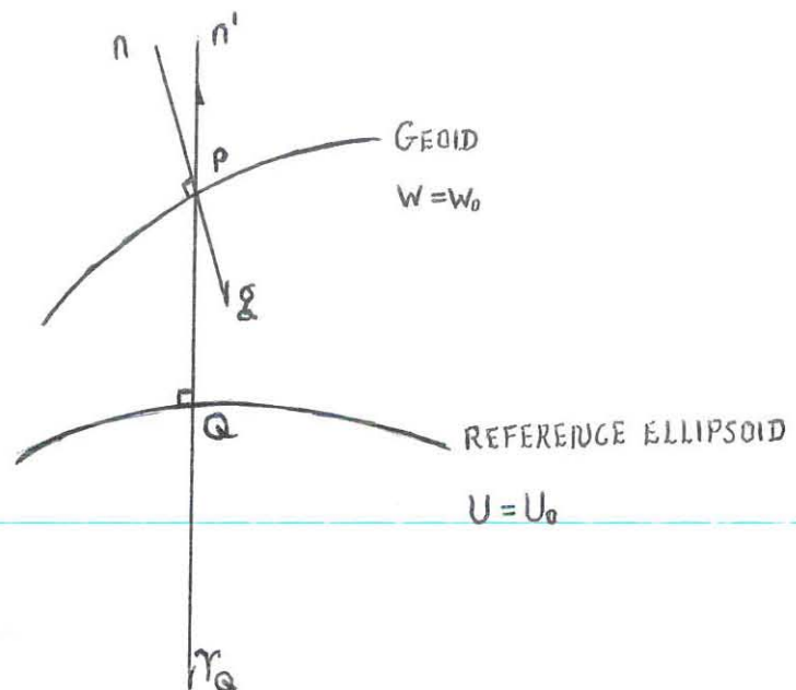
Fig.7 Geoid and reference ellipsoid. n and n' are the unit normals to the geoid and ellipsoid respectively.
