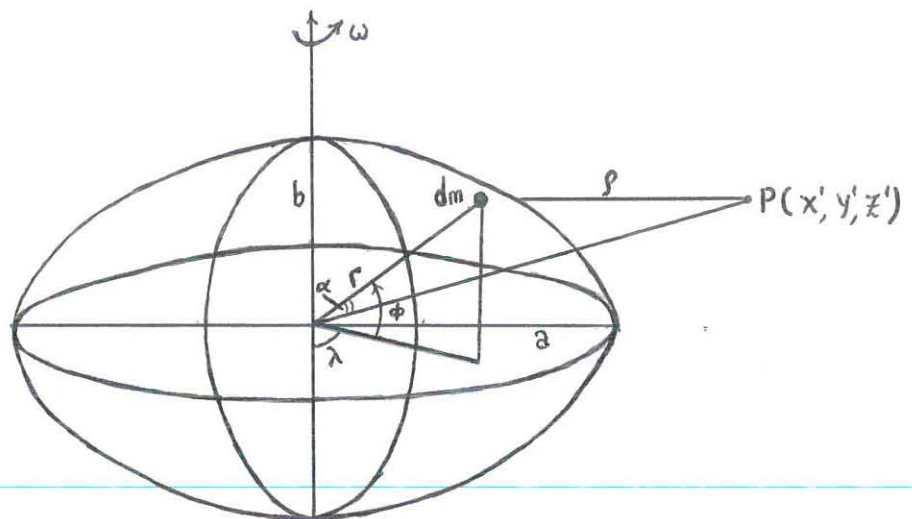
Fig.5 The components of the gravity force: attractive ( F ) and centrifugal ( f_{cg} ) force, assuming a rotating spherical Earth.
