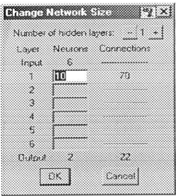
Figure 6: Screen for Network size in BrainMaker
