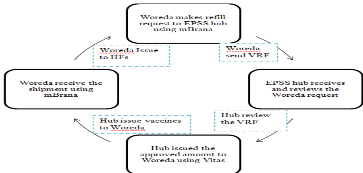
Figure2.1. mBrana information flow
