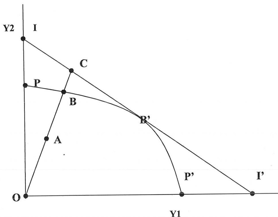
Figure 3.2 Technical and Allocative Efficiencies from Output-Orientation
