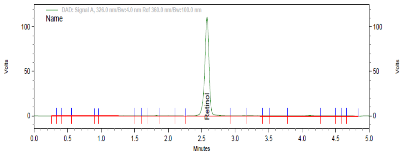
Figure 6. Chromatogram of vitamin A determination in oil sample
