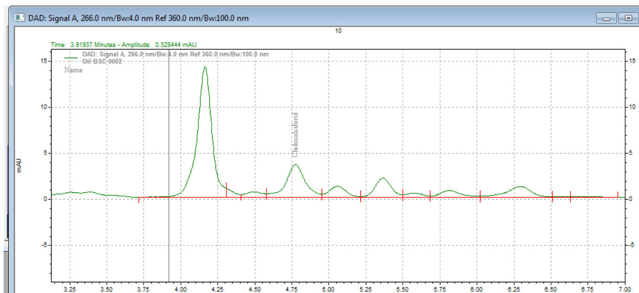
Figure 7. Chromatogram of vitamin D 3 determination in oil sample
