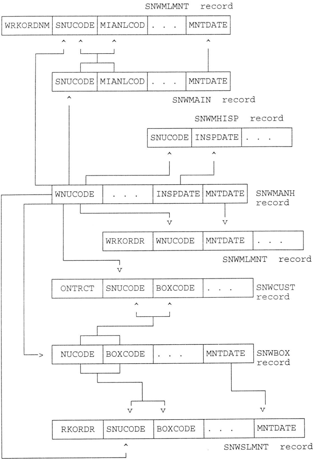
Figure 4.15: Structure of SNIS Database
