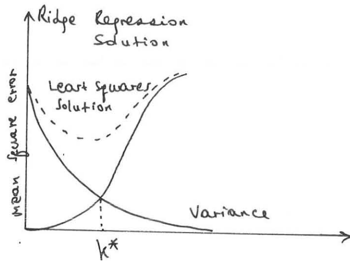
Fig. 3. Mean square error functions for the Ridge Regression estimator
