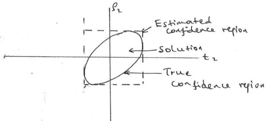
Fig.4 Hypothetical solution space for a thin conductive layer.
