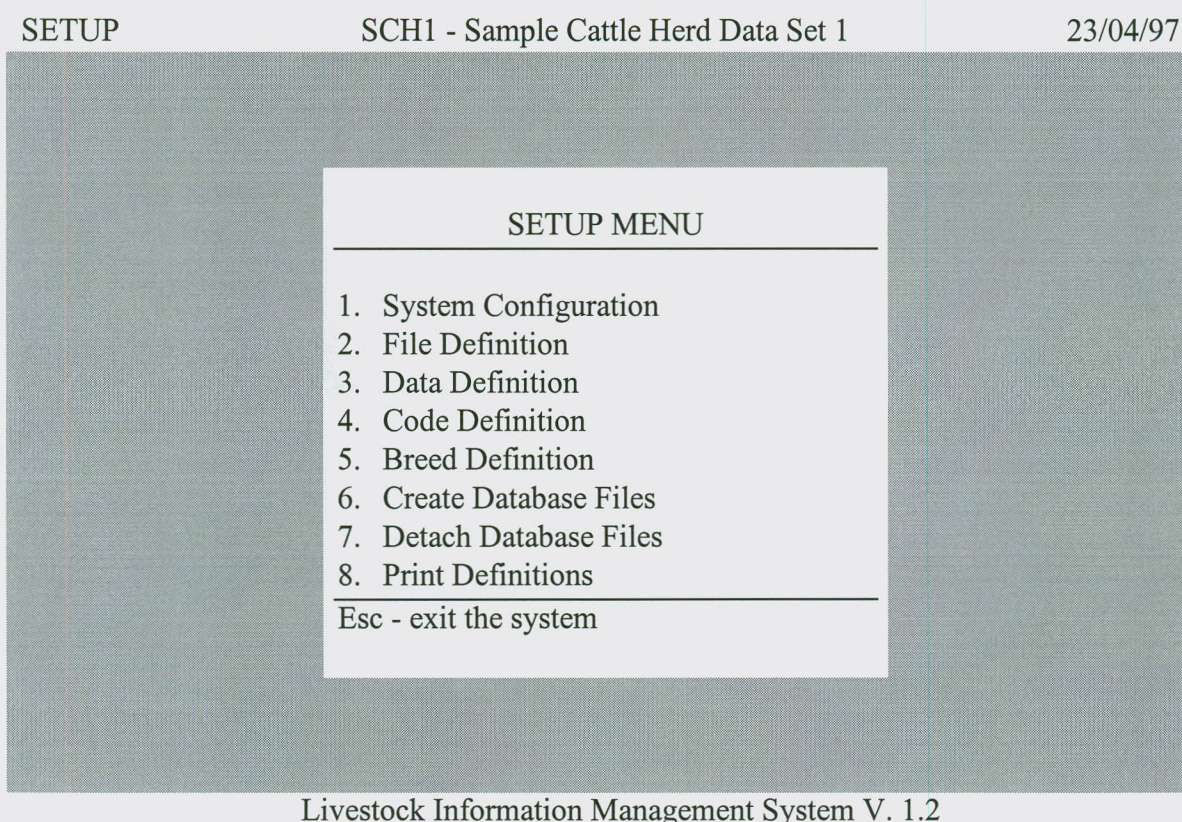
Figure 3.1 SETUP Menu Options
