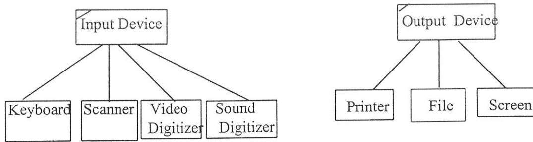
Figure 4.13 Inheritance Hierarchy of Input and Output devices (Interface Subsystem).
