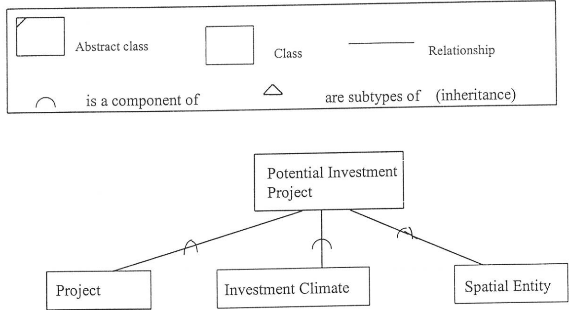
Figure 4. 8 Composed of Hierarchy of Potential Investment Project Subsystem
