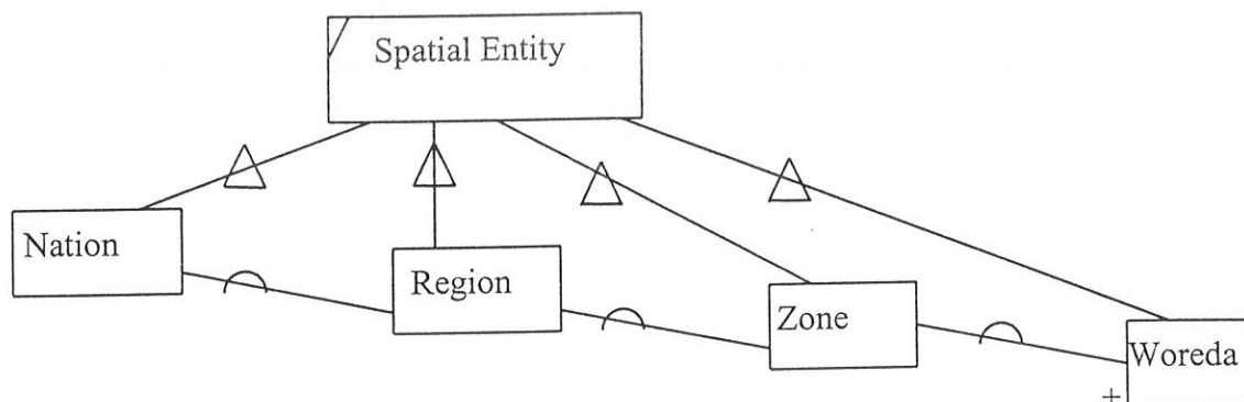
Figure 4.9 Hierarchical Diagram of Spatial Entity. "+" indicates that further sub-classification may be required.
