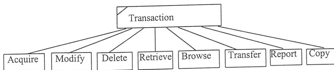
Figure 4.12 Inheritance Hierarchy of Transaction.
