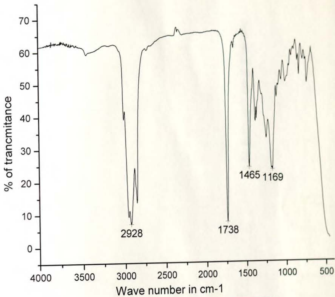
Appendix 2: IR spectrum of VG-3
