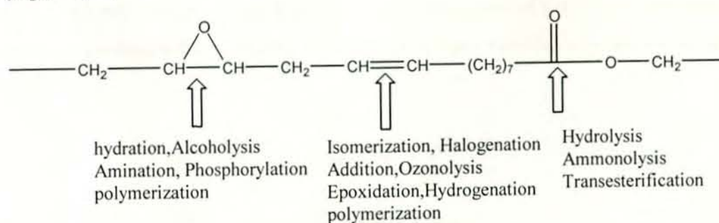
Fig 4. A wide variety of reaction characteristics of epoxy acid within the triglyceride
