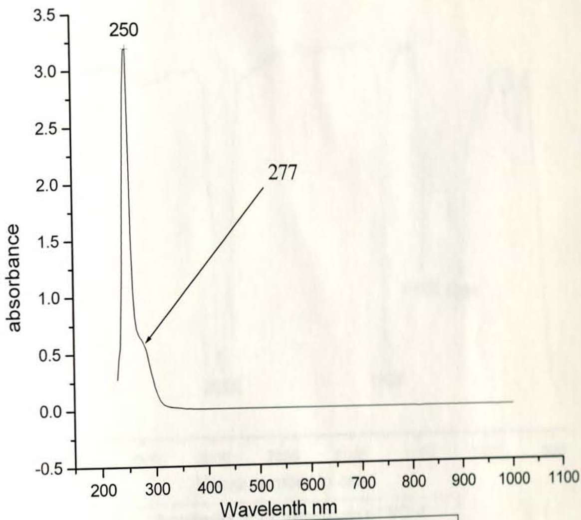
Appendix 1: UV-Vis spectrum of VG-3
