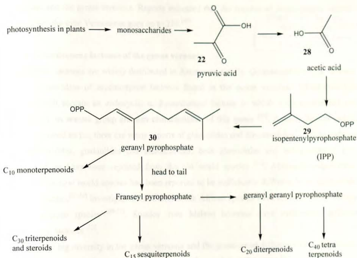
Figure 9. Biosynthesis and biogenic relationships of terpenoids.
