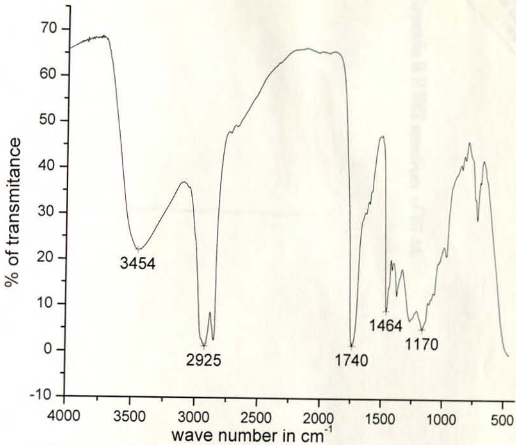
Appendix 9: IR spectrum of VG-4A
