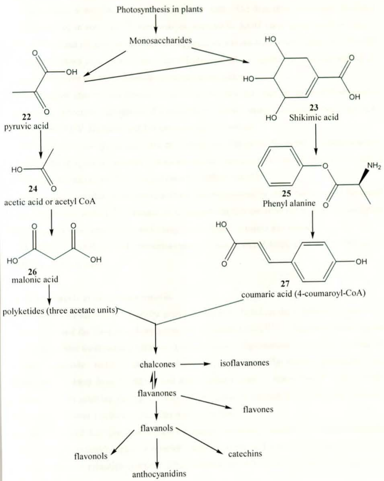
Fig 8: Biosynthesis and biogenetic relationships of flavonoids
