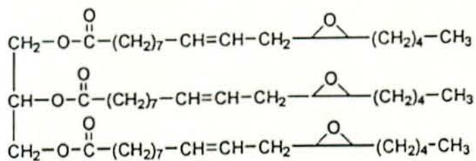
Figure 2. Structure of trivernolin
