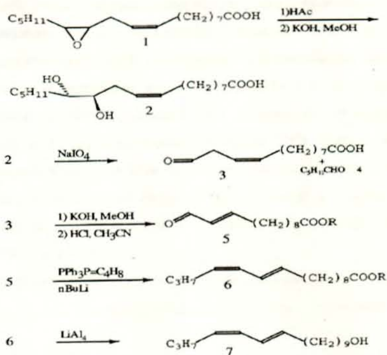
Fig 5. Synthetic route from vernolic acid to bombykol
