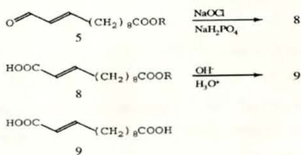
Fig 6. Synthesis of traumatic acid from the vernolic acid-derived intermediate 12-oxo-10-E-dodecenoic acid.
