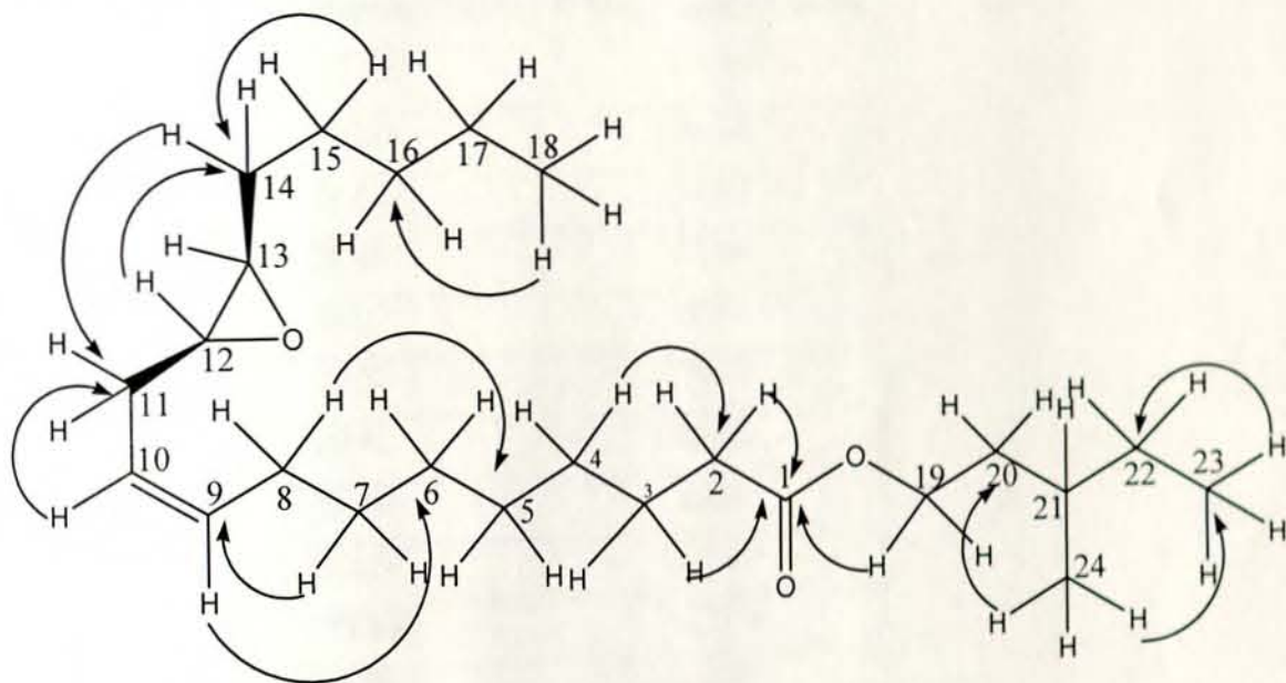
Fig. 10. The Selected HMBC Correlation of VG-3
