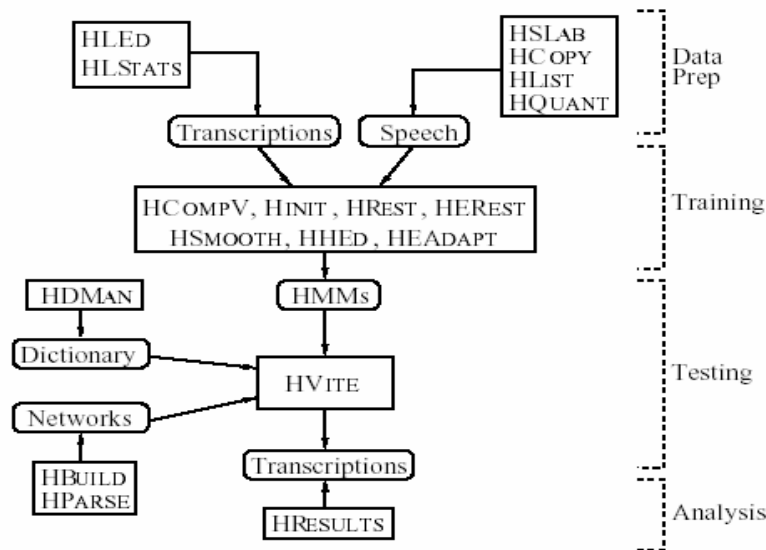
fig. 4.2. HTK processing stages (extracted from Young et. al. 2002)
