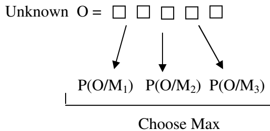
fig.2.1. Using HMM for isolated word recognition (adapted from Young et.al. (2002)).
