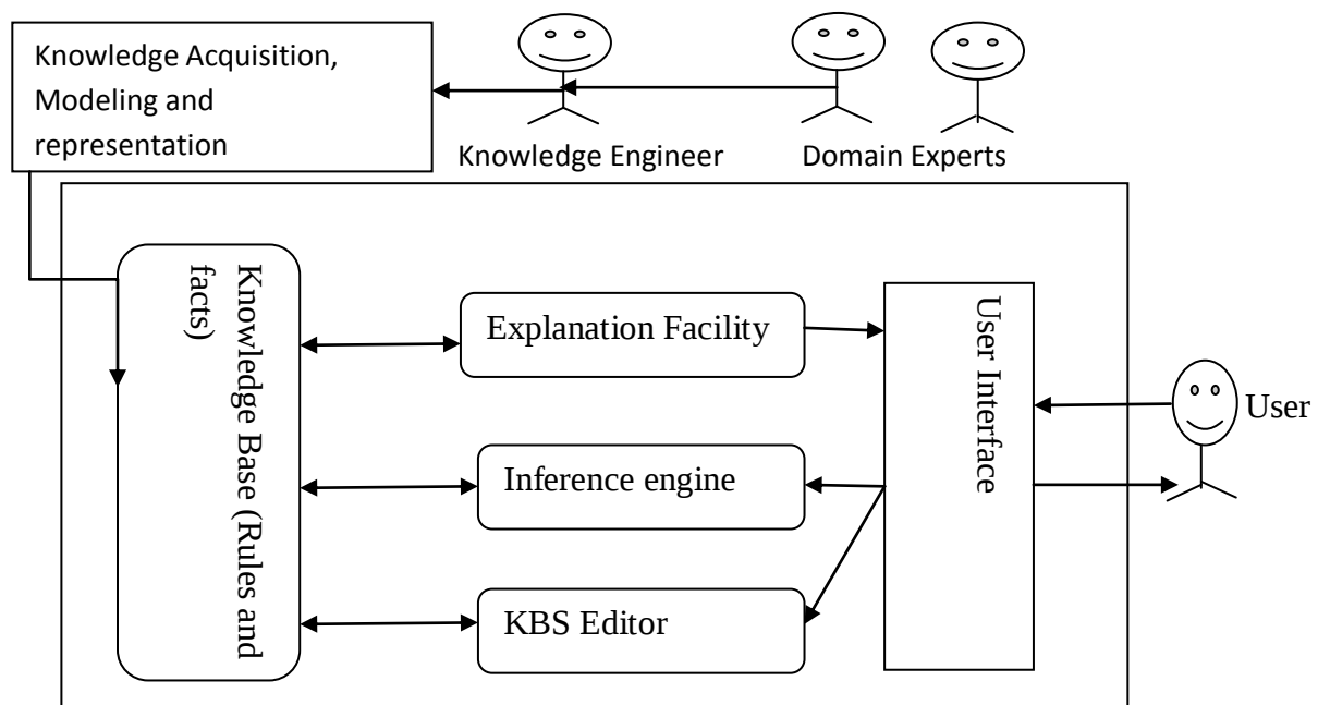
Figure 22: Architecture of the System
