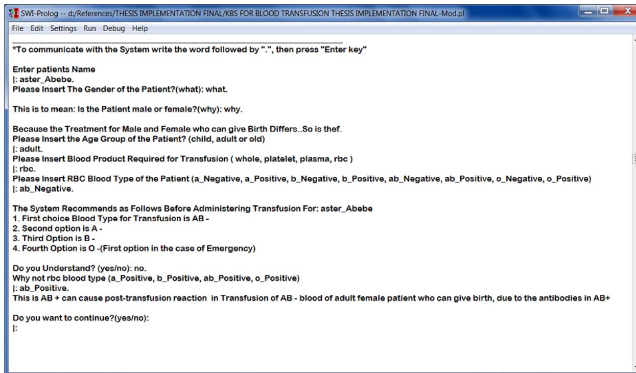
Figure 23: Sample Inferencing Dialog Between the system and the User
