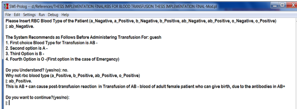
Figure 24: Samole Dialog of "WHY-NOT" Explanation Facilities
