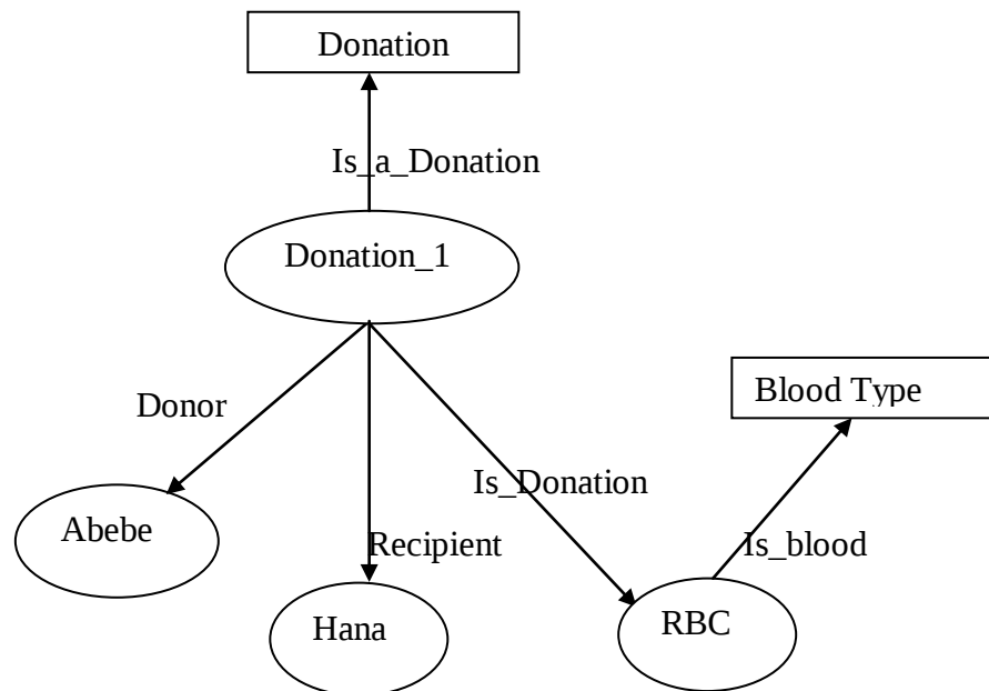
Figure 3: Semantic Net Examples
