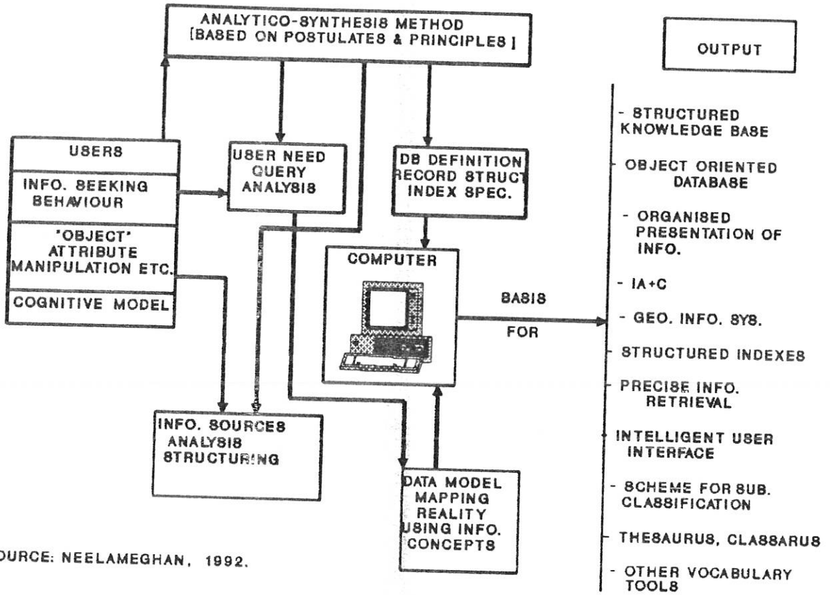
Figure 13: OODB DESIGN PROCESS
