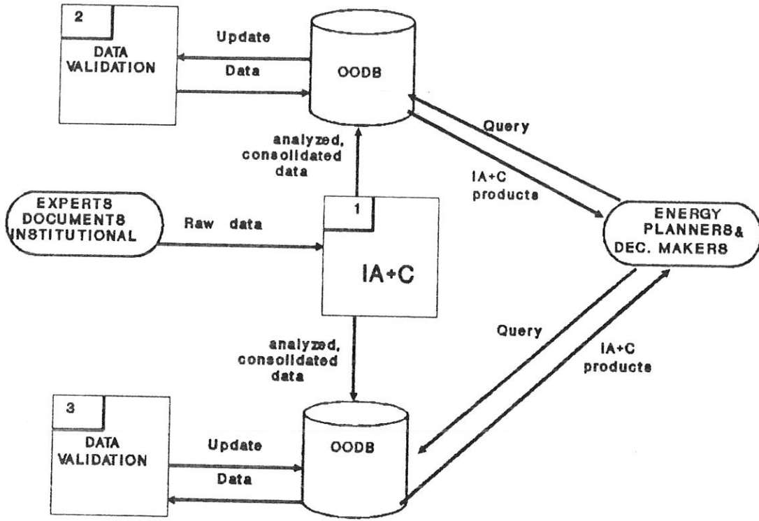
Figure 15: DATAFLOW DIAGRAM FOR ENERGY OODBS
