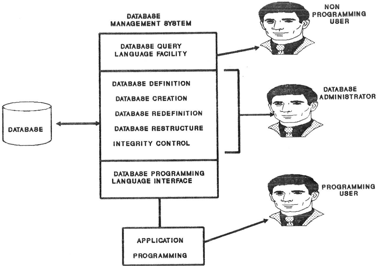
Figure 5: CONCEPTUAL MODEL OF DATABASE MANAGEMENT SYSTEM
