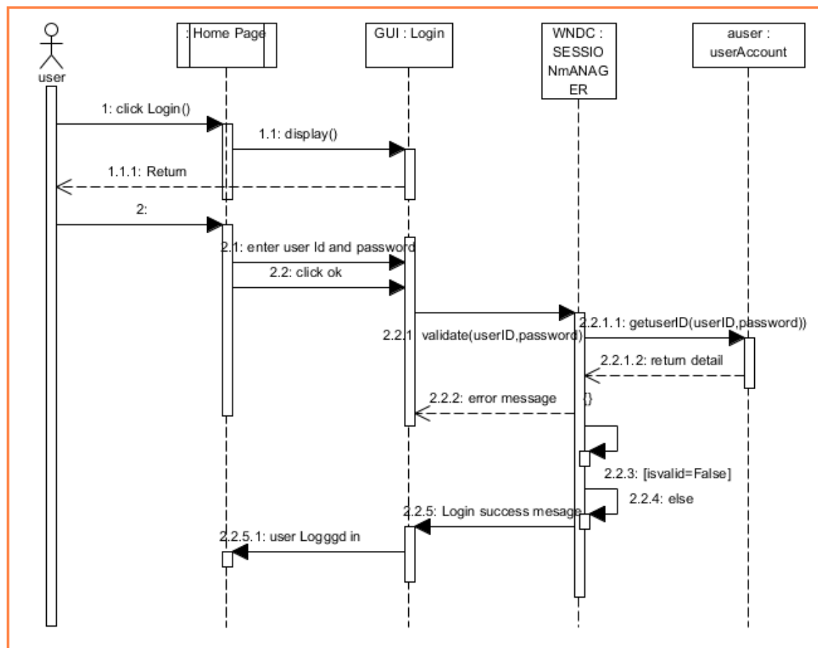
Figure 13:- Sequence diagram for Login use case
