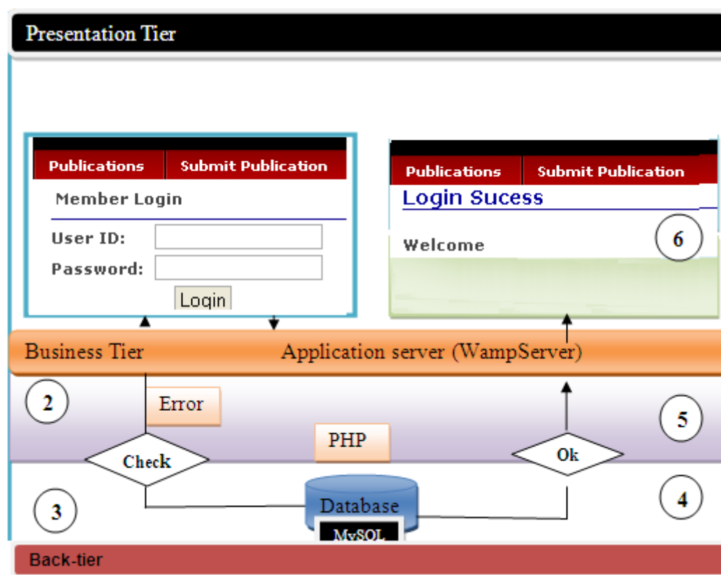
Figure 4: The Three-Tier Architecture of the WNDC System
