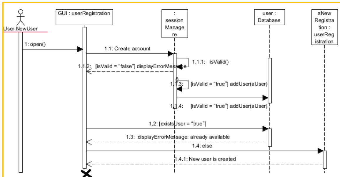
Figure 14:- Sequence diagram for user registration use case
