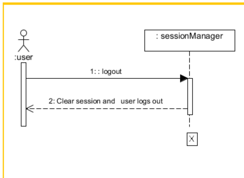
Figure 15:- Sequence diagram for Logout use case
