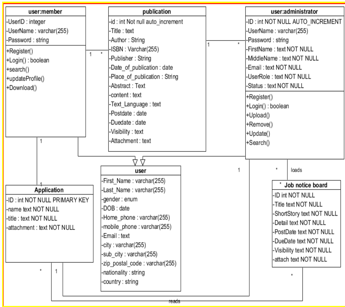
Figure 19: Class diagram of WNDP
