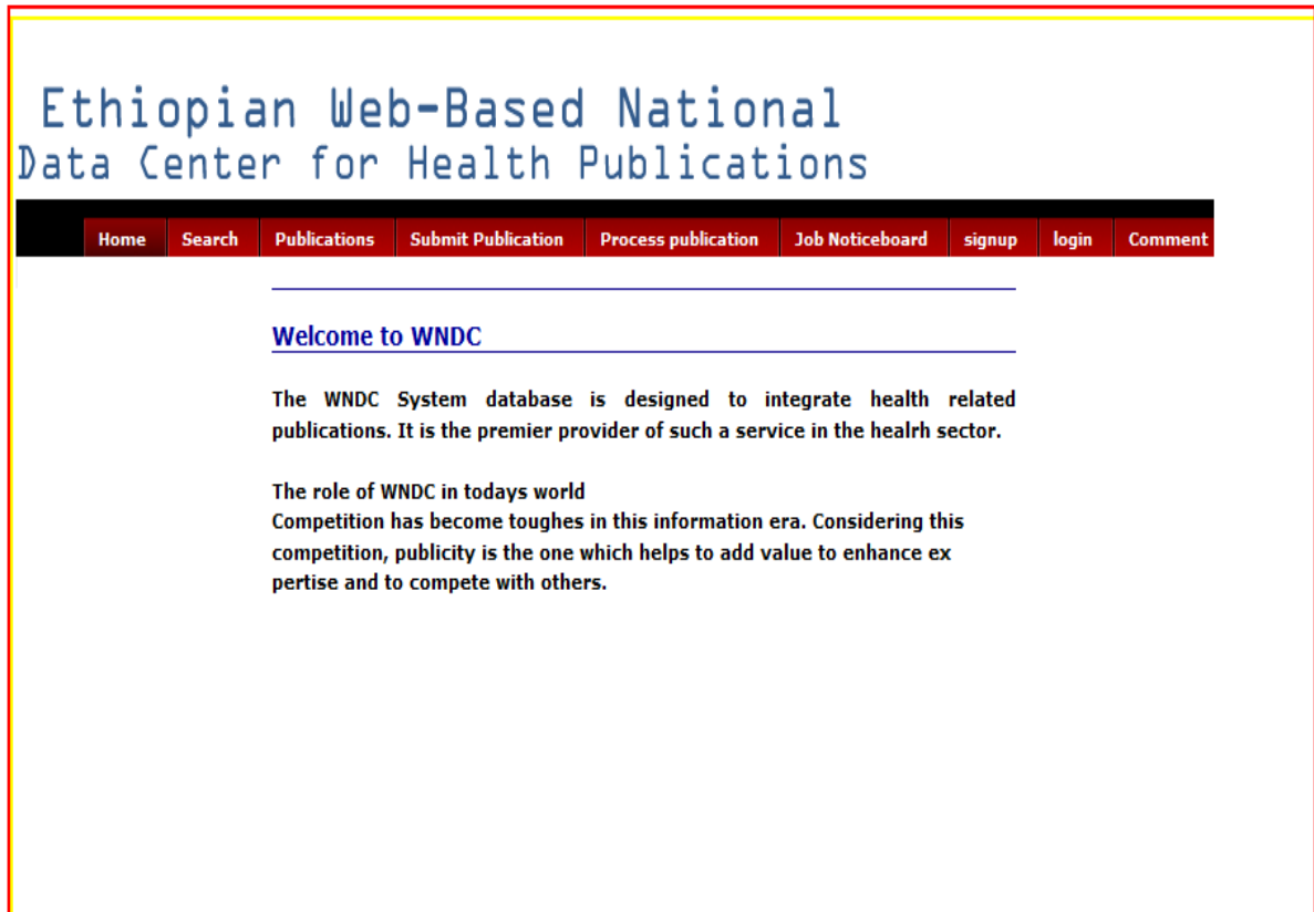
Figure 5: Index Page
