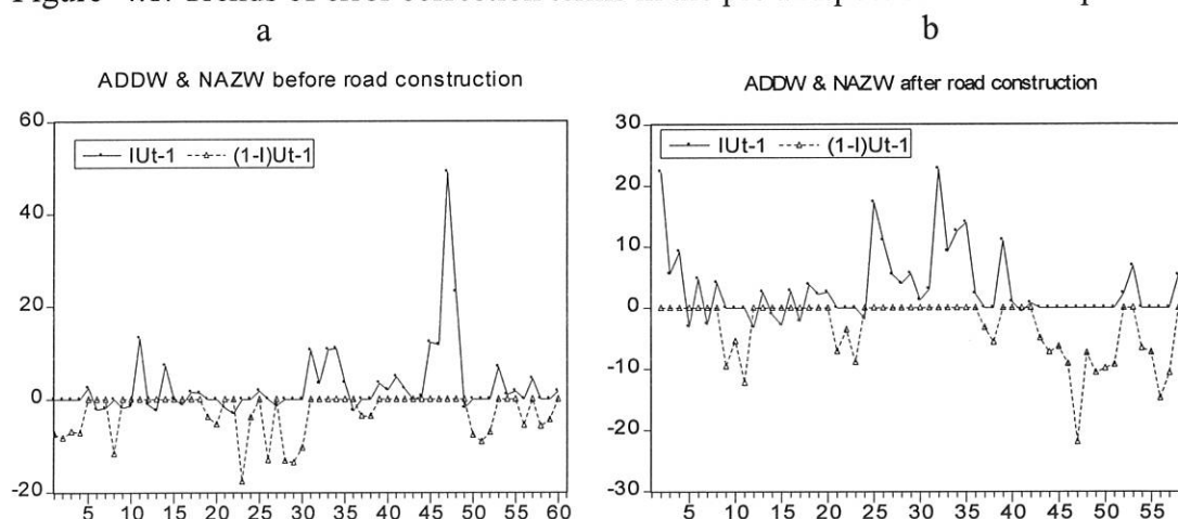
Figure 4.1. Trends of error correction terms in the pre and post construction period
