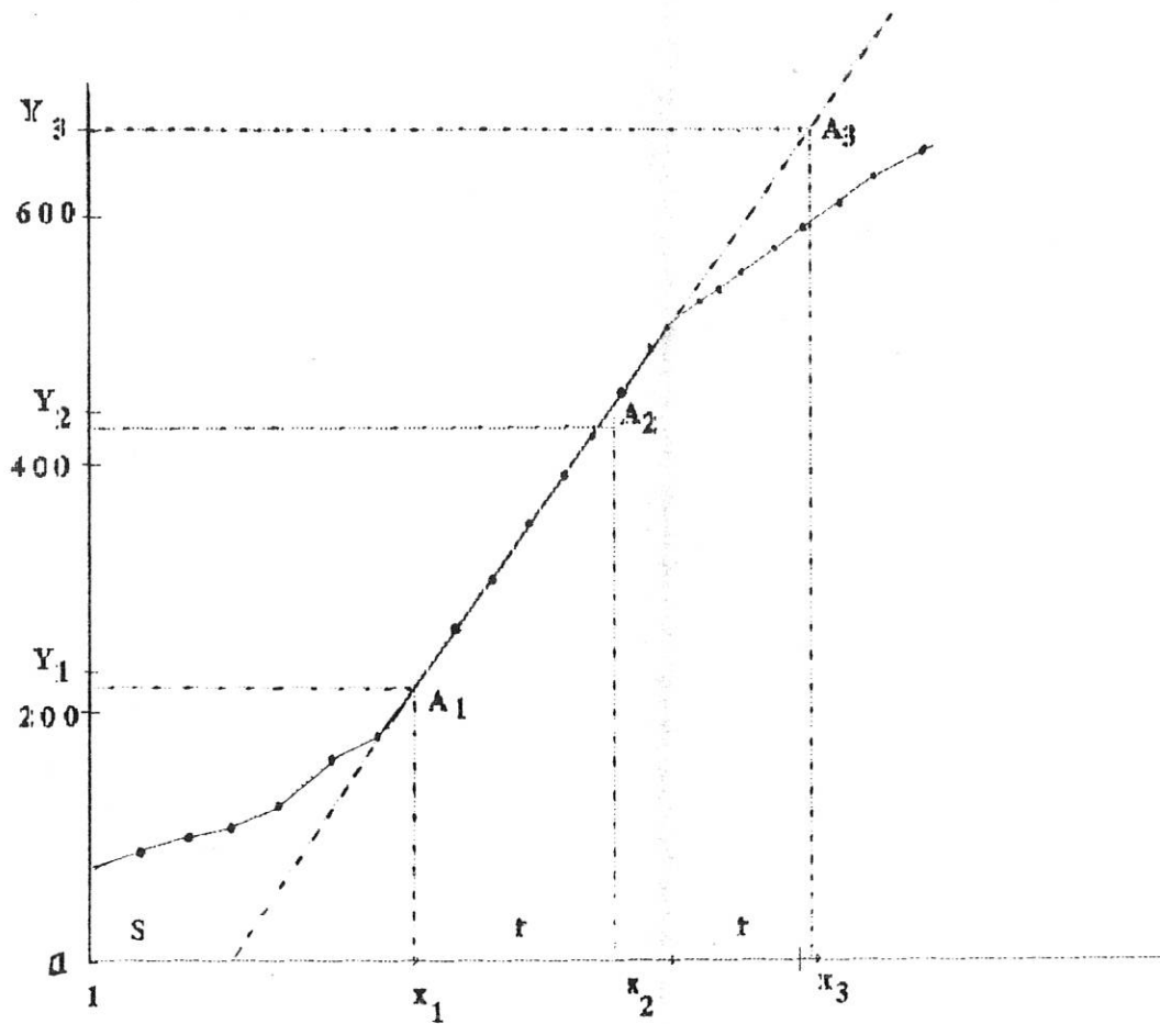
Fig. 3.1 Bradford Curve
