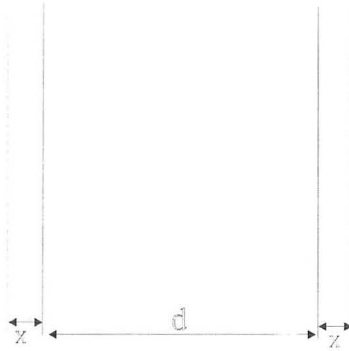
Figure 3.1: Displacement of a slab of charge.
