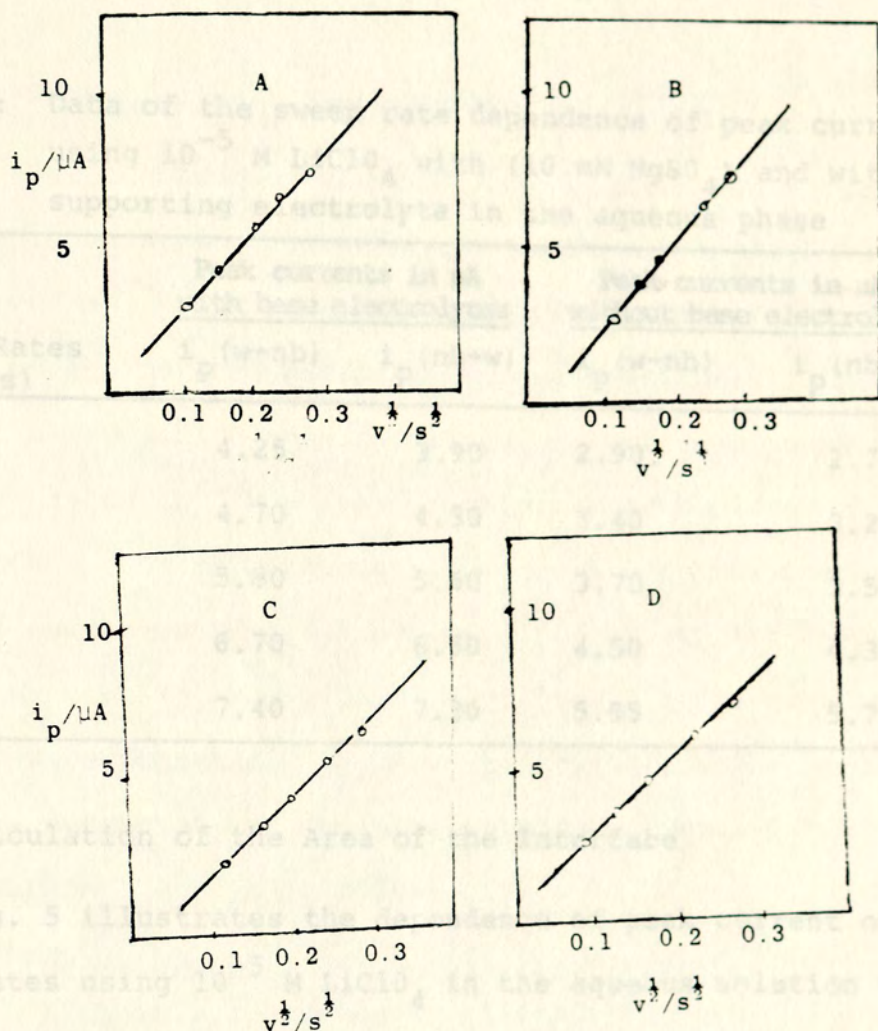
Fig. 4: The dependence of peak currents, i_p , on the square root of polarization rate, v , using 10^{-5} M LiClO_4 with (A, B) and without (C, D) supporting electrolyte in the aqueous phase ( 10 mM M SO_4 ). Curves A and C corresponds to the transfer of ClO_4^- ion from the aqueous to the organic phase while B and D corresponds to the opposite transfer, i.e. from organic to aqueous. In all cases the organic phase contains 10 mM CVTPB as base electrolyte.
