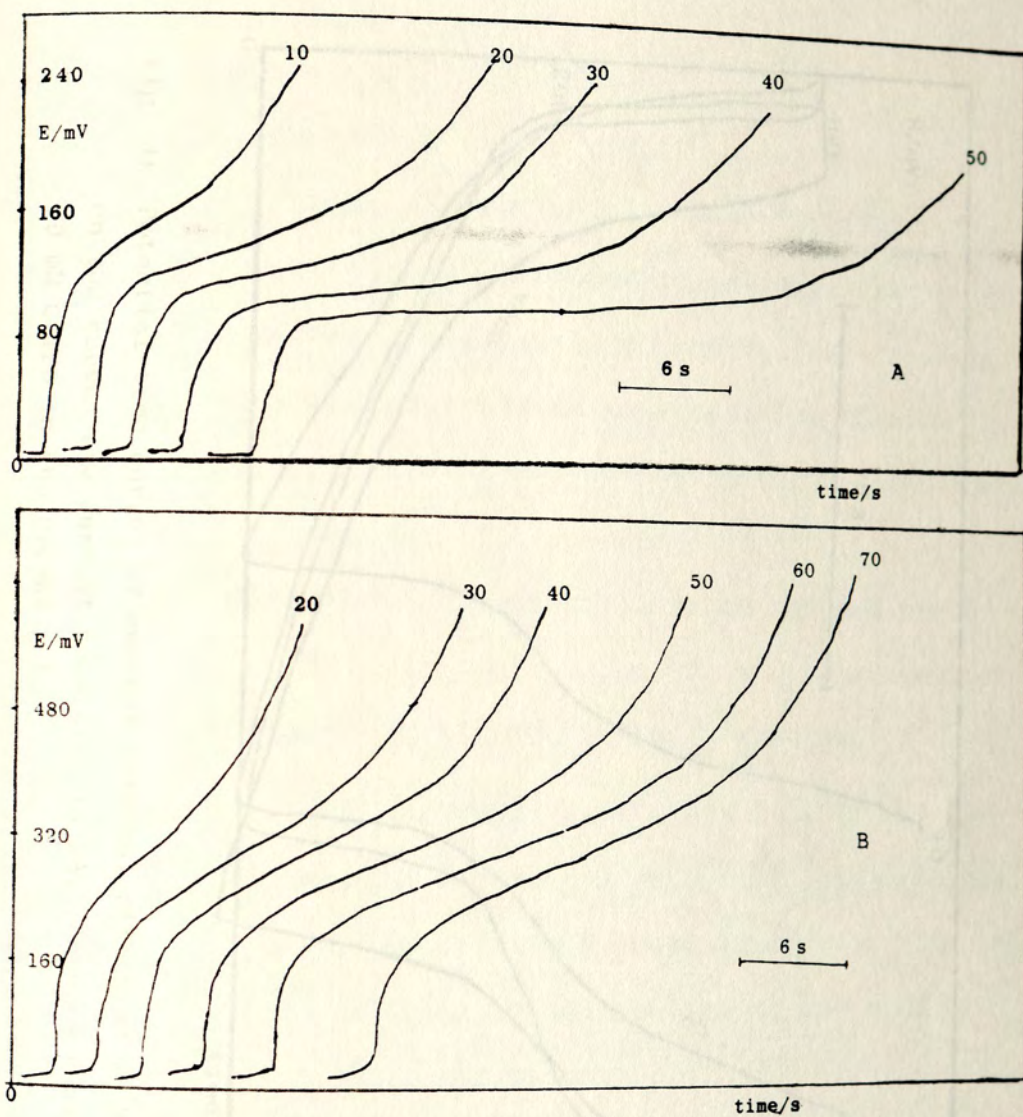
Fig. 8: PSA (potential-time curves) of 10^{-5} M \text{LiClO}_4 (A) in a quiescent solution and 10^{-4} M \text{KNO}_3 (B) in a stirred solution which is agitated at a rate of 1500 r.p.m. Aqueous phase: 10 mM \text{MgSO}_4 and organic phase: 10 mM CVTPB in the PVC-nb gel.
