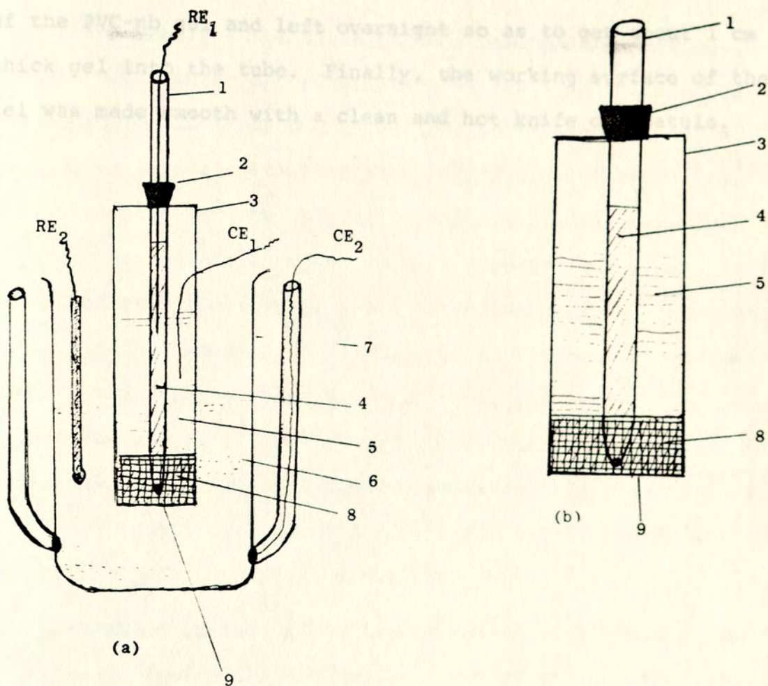
Fig. 1: Electrochemical cell setup (a), polyvinylchloride-nitrobenzene gel electrode (b). Ag/AgCl/Cl - reference electrodes (RE 1 , RE 2 ), silver wire counter electrodes (CE 1 , CE 2 ), glass capillary tube (1), silicon rubber (2), polytetrafluoroethylene (PTFE) tube (3), 0.1N KCl solution (4), 10 mM M g SO 4 solution (5); PVC-nitrobenzene phase (8), working interface (9), aqueous solution (6), glass beaker (7).
