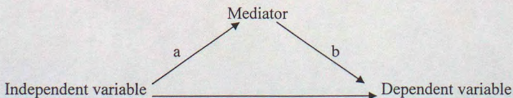
Mediation Model
