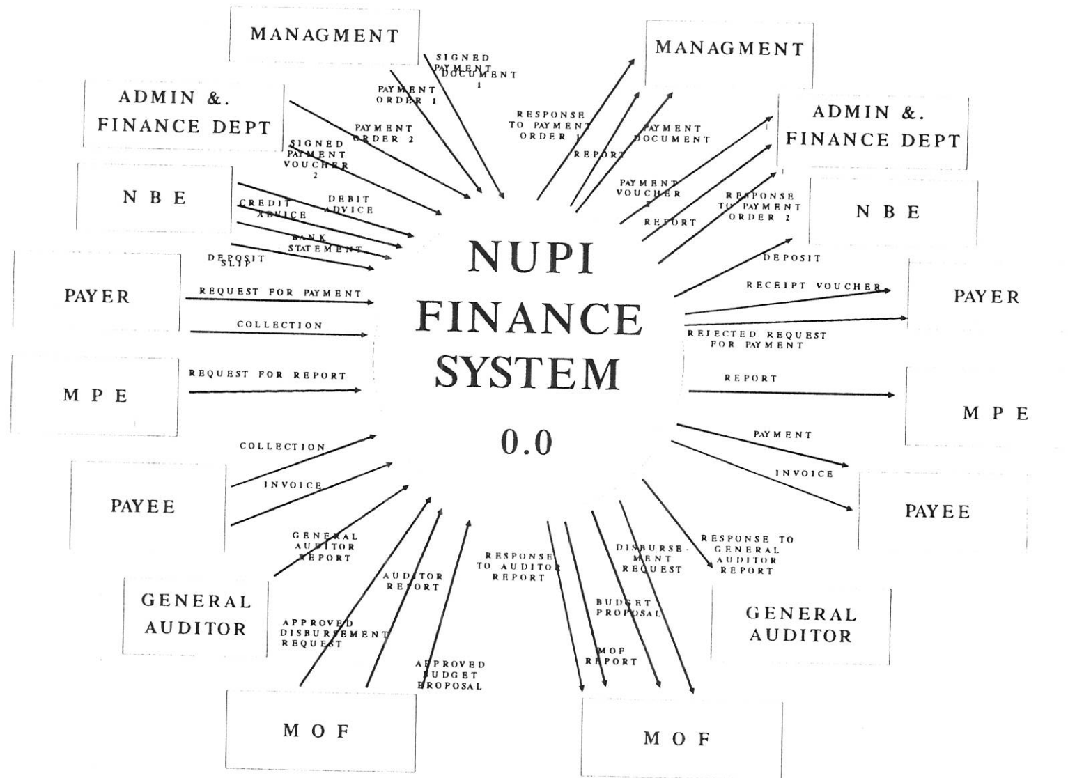
FIG 2.1 CONTEXT DFD OF NUPI FINANCE SYSTEM NOTE: Two entities with same name are considered as one entity.
