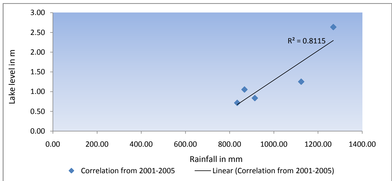
c. Correlation between mean annual rainfall and lake level from 2001-2005
