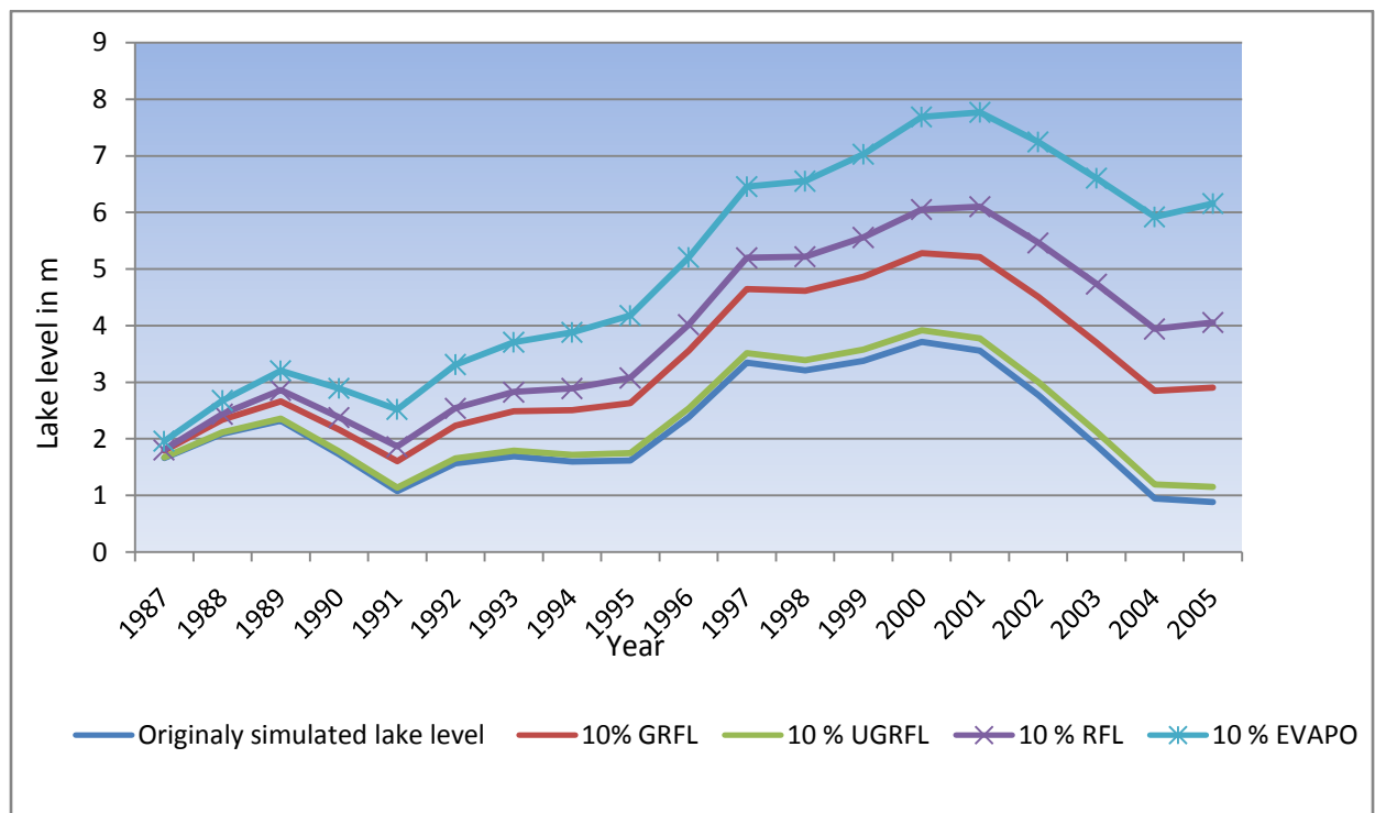
Figure 6 7 A simple sensitivity analysis to the variables by adding a 10% increase from their base period average values
