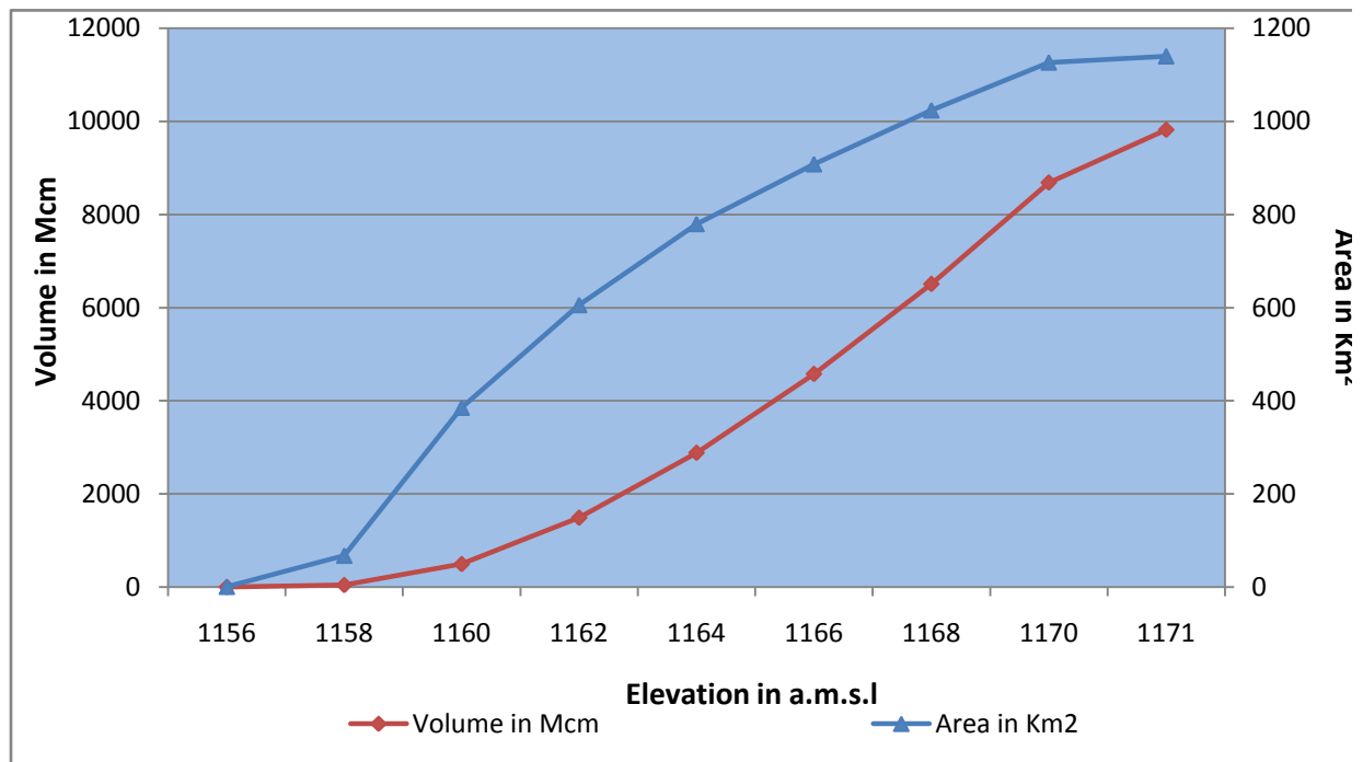
Figure 6 2 Area-Capacity Curve of Lake Abaya
