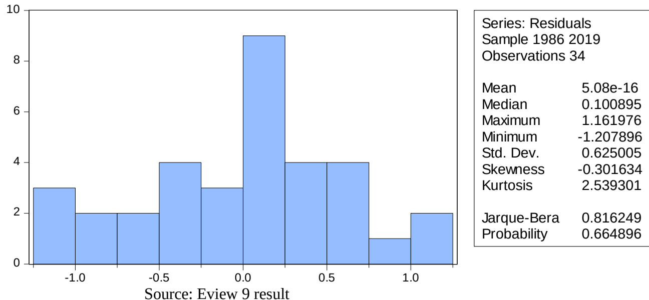
Figure 5. 1 normality test
