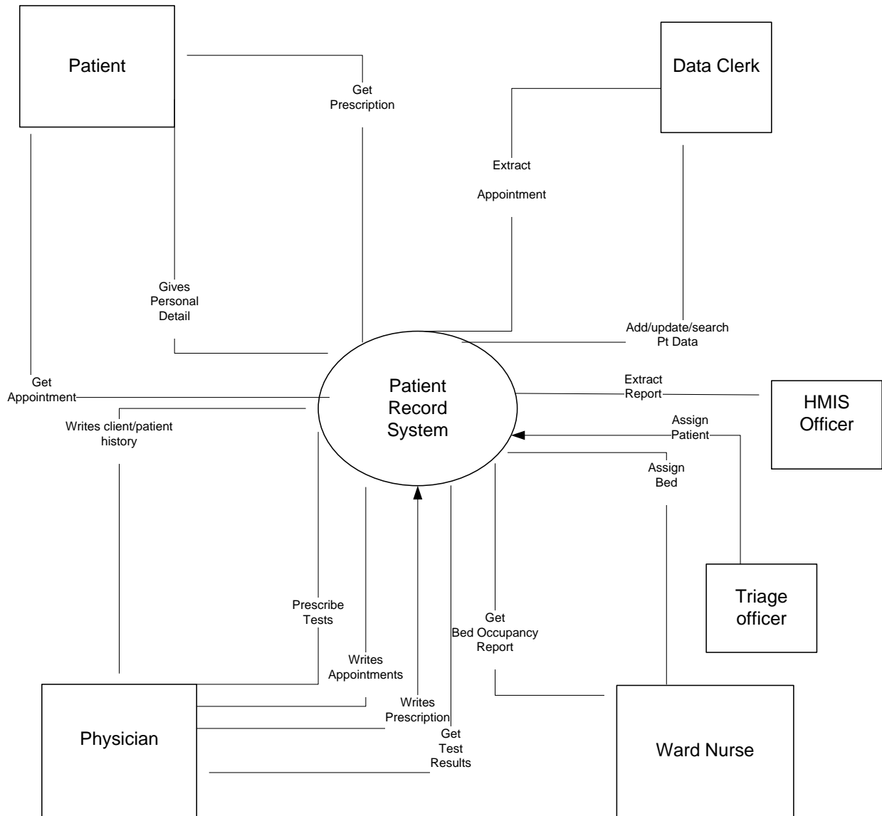
Fig 8: Context Diagram of a Patient Record System
