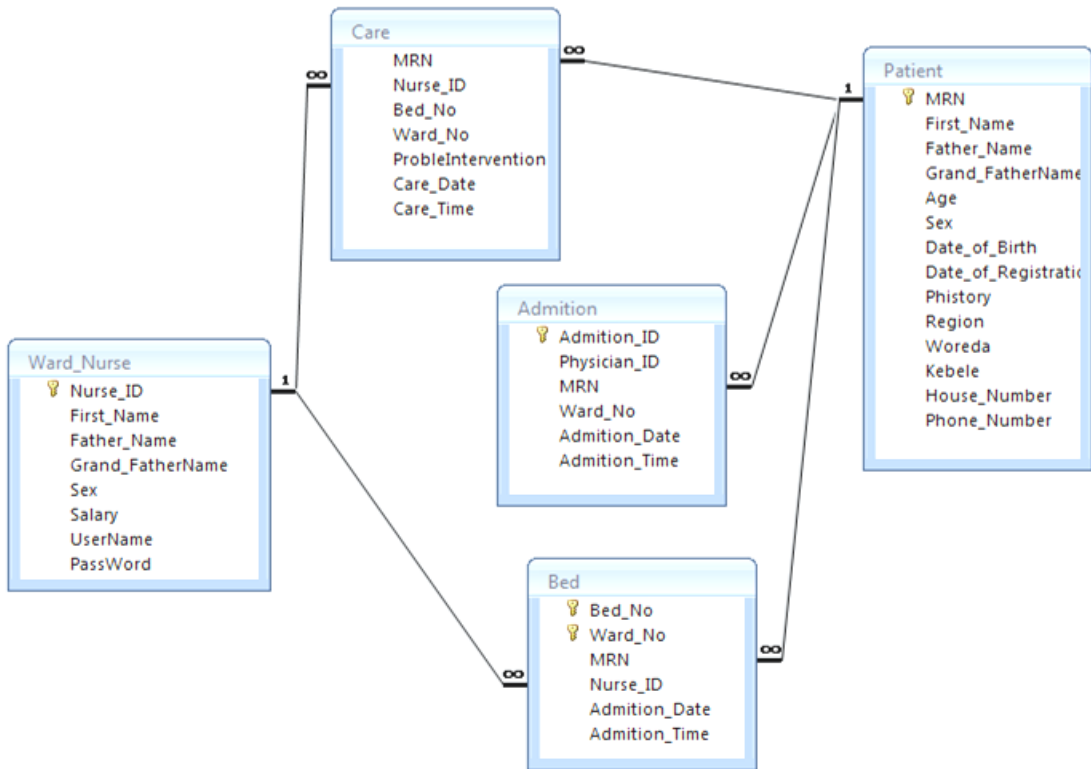
Fig 19: ER Diagram of Patient and Ward Nurse
