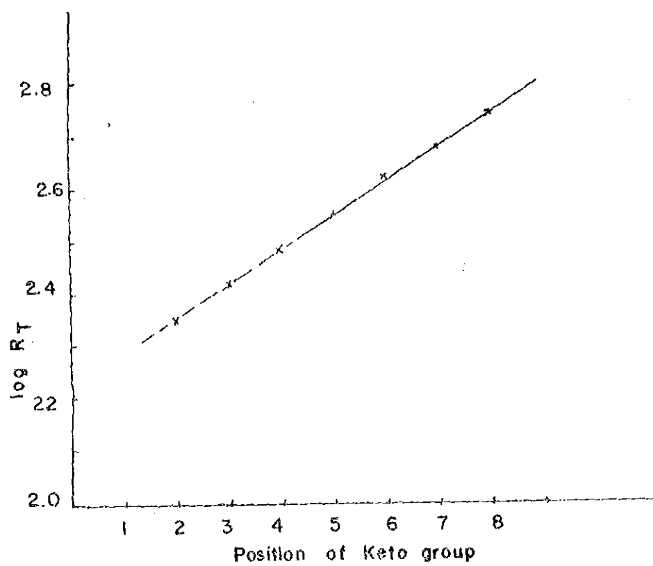
Fig. 1: \log R_T VS Position of Keto group
