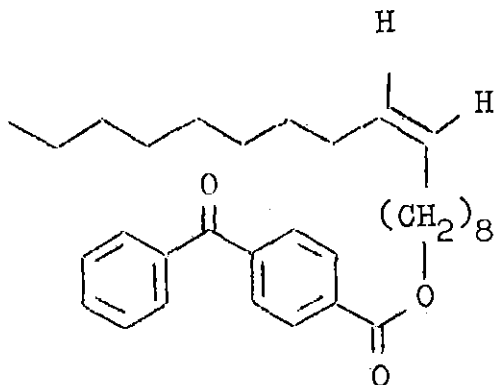
Oleyl ester of p-benzoylbenzoic acid
