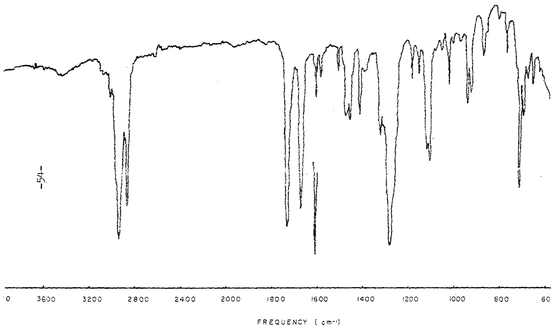
Ir Spectrum of OLEYL ESTER of P-BENZOYLBENZOIC ACID (ester I)
