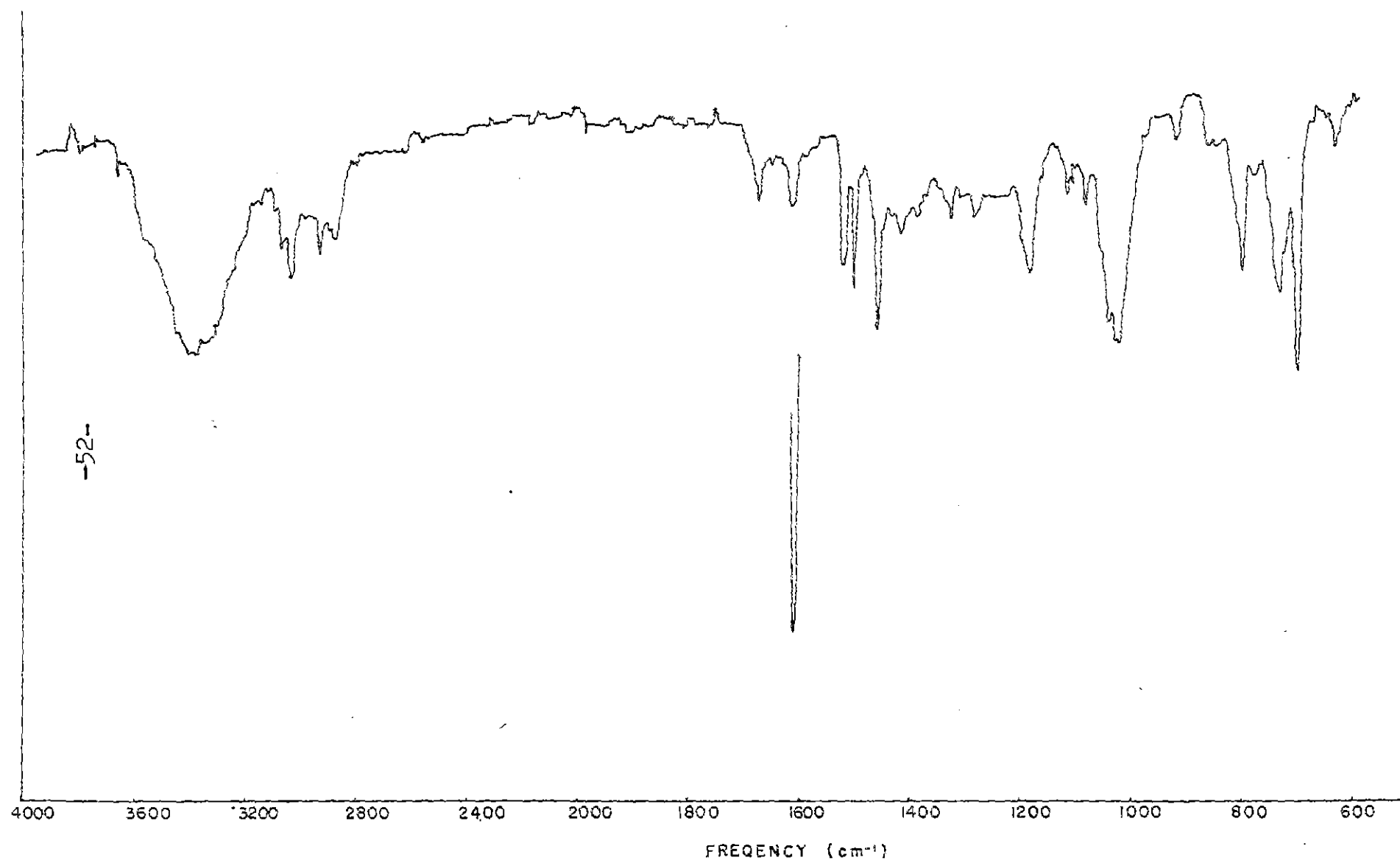
Tr Spectrum of PHENYL-P-TOLYL CARBINOL (20)
