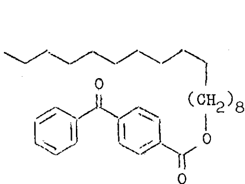
Stearyl ester of p-benzoylbenzoic acid
