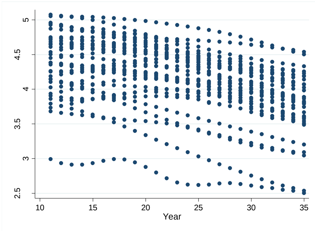
Figure A1: Scatter plot of infant mortality over time
