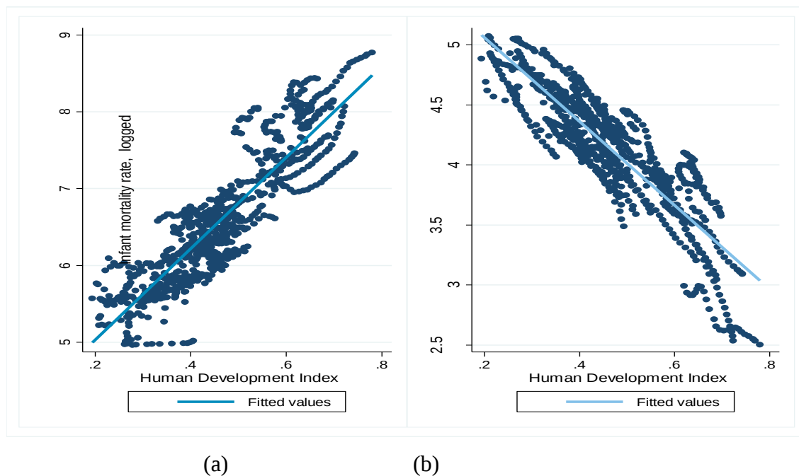
Figure 3.2. Scatter plots of household consumption per capita and infant mortality rate versus HDI over 1990-2014 for 40 African countries
