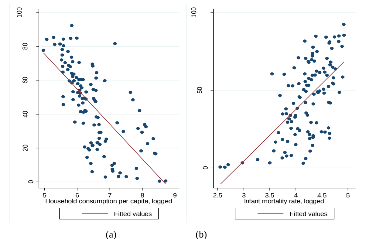
Figure 3.1. Scatter plot and fitted value of poverty headcount ratio at $1.90 per day versus the log of household consumption per capita and the log of infant mortality rate in panels (a) and (b) respectively across African countries for various years in 1980-2014
