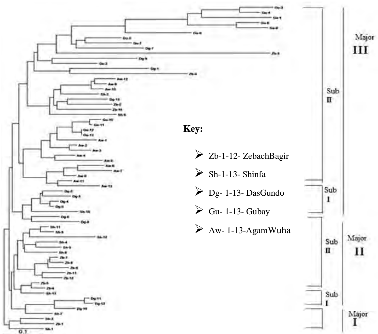
Figure 5 Neighbor-joining analysis of 64 individuals based on 39 PCR bands amplified by five primers. The neighbor joining algorithm is based on Jaccard's coefficients obtained after pair wise comparison of the presence-absence fingerprint.
