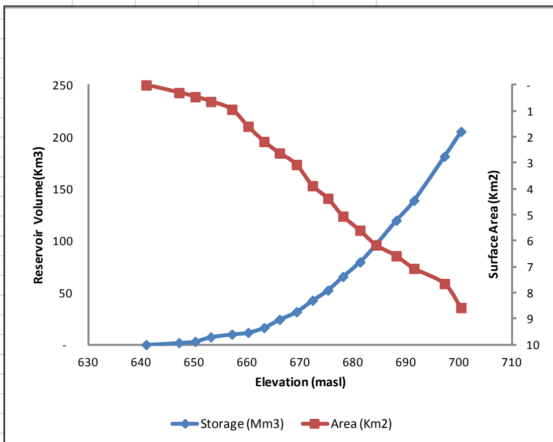
Figure 3-6 Elevation-Storage-Area Curves for GD-5 Reservoir
