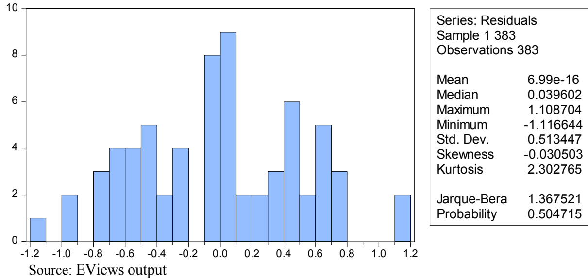
Figure 4.7.5 Normality Test
